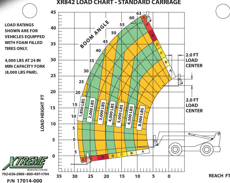
XR842 LOAD CHART - STANDARD CARRIAGE
