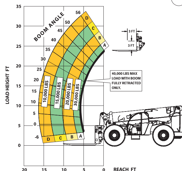
XR4030 LOAD CHART - FORK POSITIONING CARRIAGE
