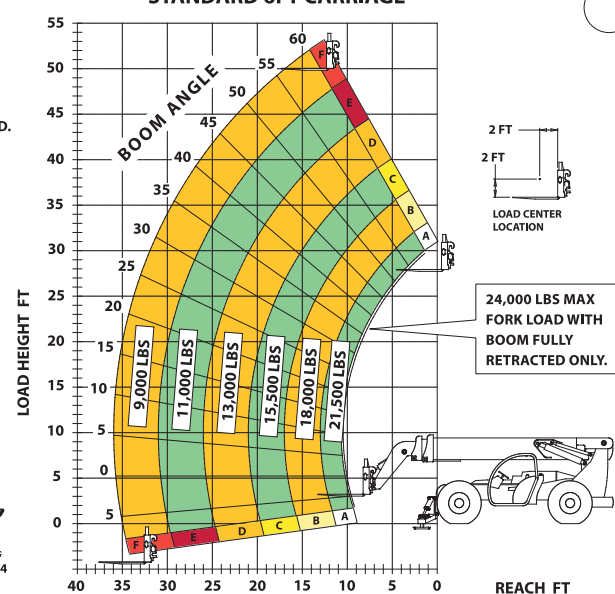
XR2450 LOAD CHART OUTRIGGERS DOWN STANDARD 6FT CARRIAGE
