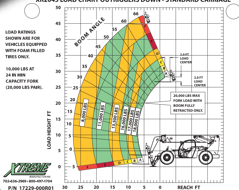
XR2045 LOAD CHART OUTRIGGERS DOWN - STANDARD CARRIAGE
