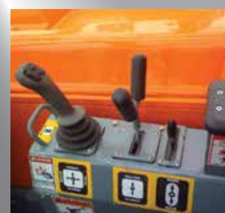
Operator Controls
