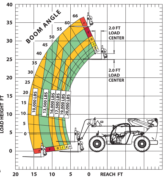
XR2034 LOAD CHART - STANDARD CARRIAGE
