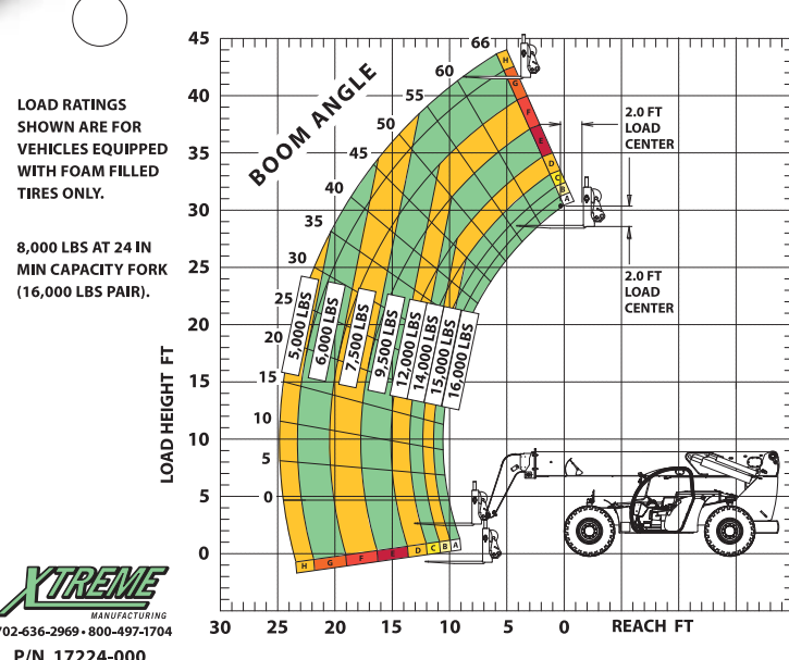
XR1642 LOAD CHART - STANDARD CARRIAGE
