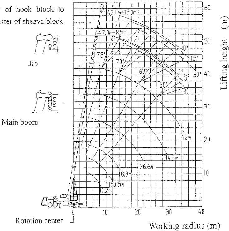
Fig. 3-2 Lifting Height Chart
