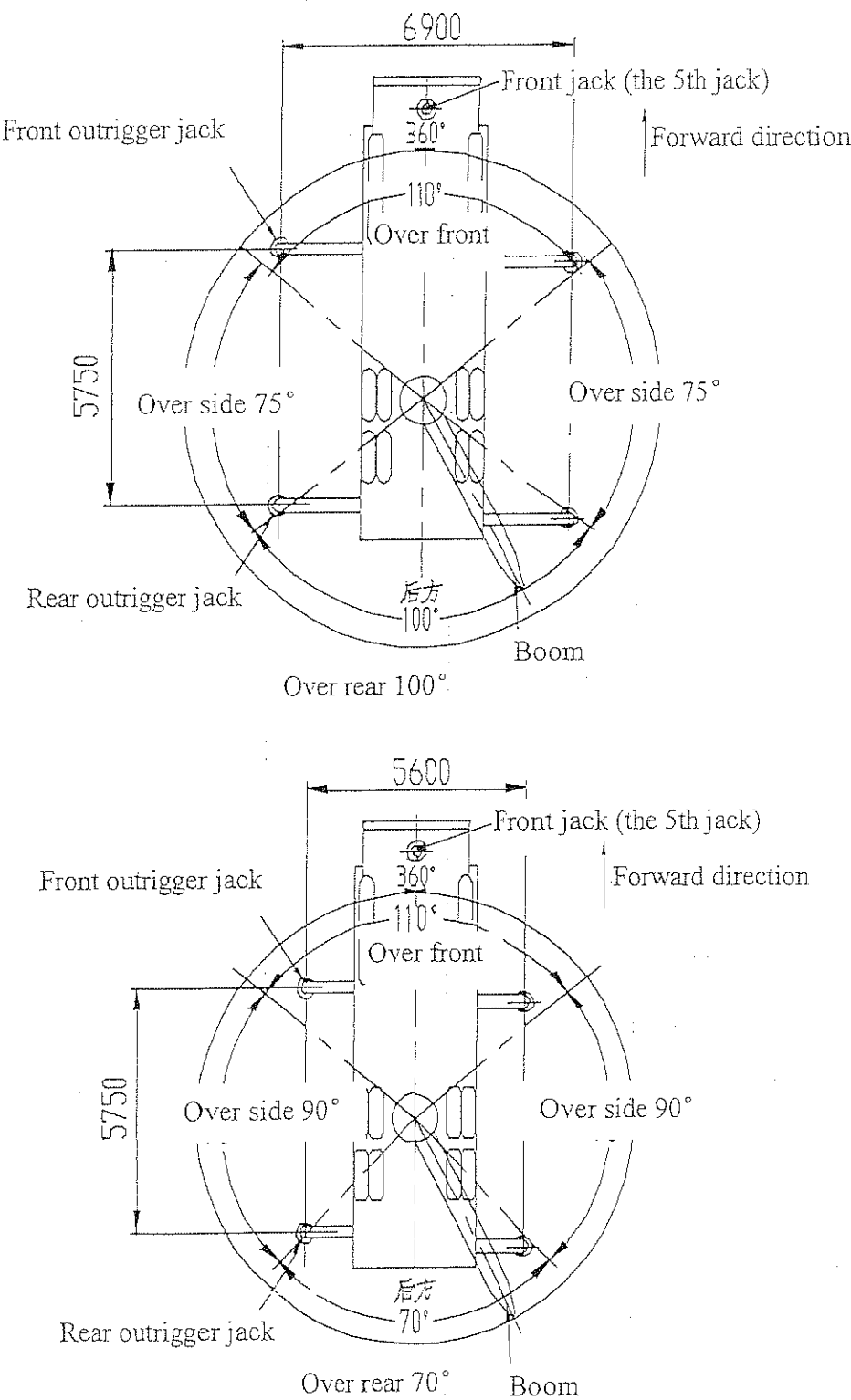
Fig. 3-3 Crane Working Areas
