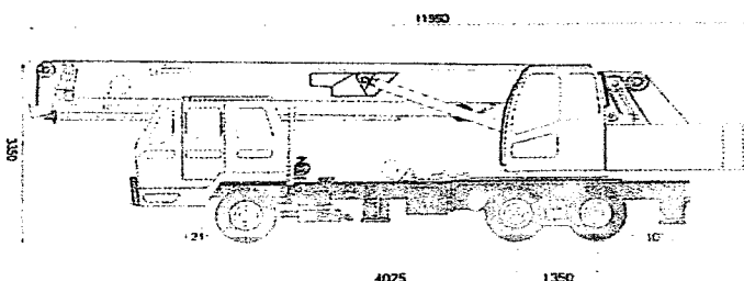
机外形尺寸 Outline dimensions
