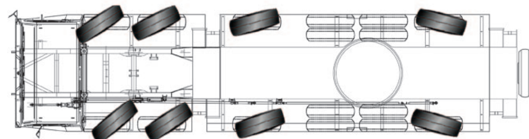
4-axle steering and 3-axle drive
