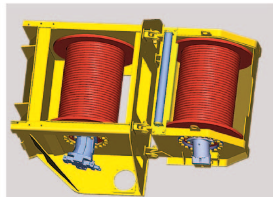
Two independently-operated winches
