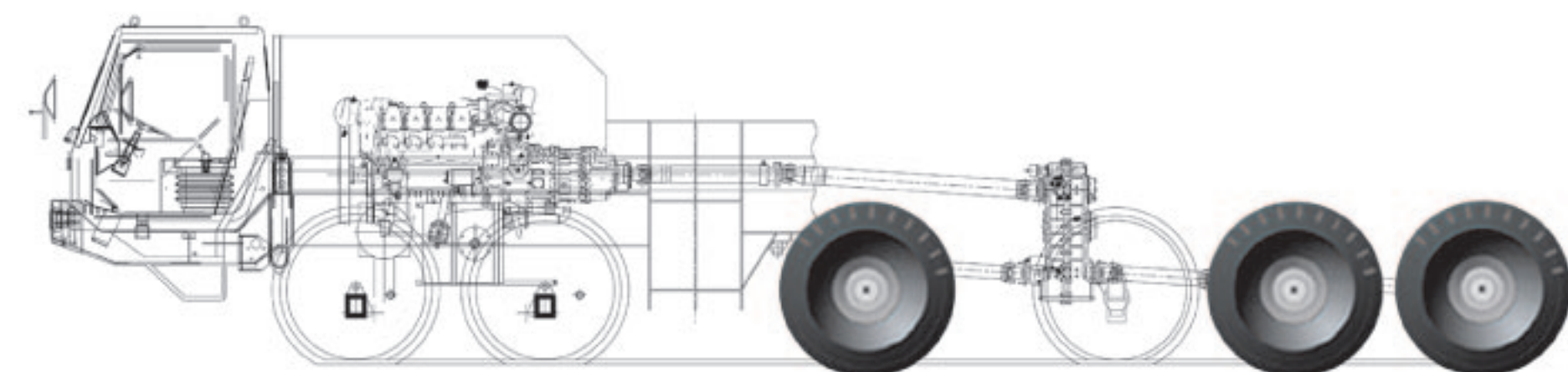
4-axle steering and 3-axle drive
