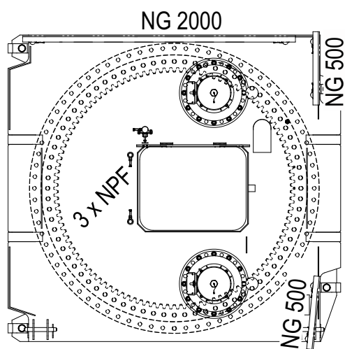
Arrangement of standard railings, slewing frame
