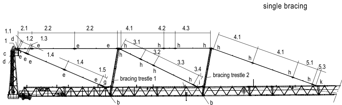
Jib brace diagram 75m - 70m
