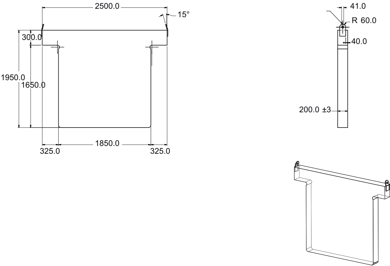
Data counterweight block 5.97 t
