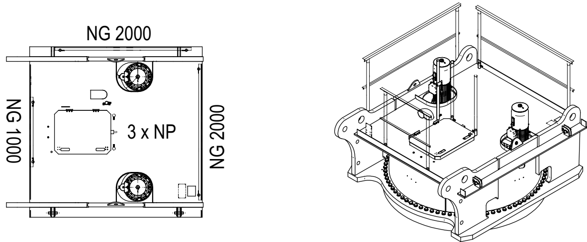
Arrangement of standard railings, slewing frame
