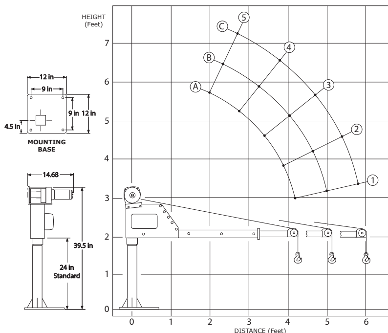
LOAD CHART
