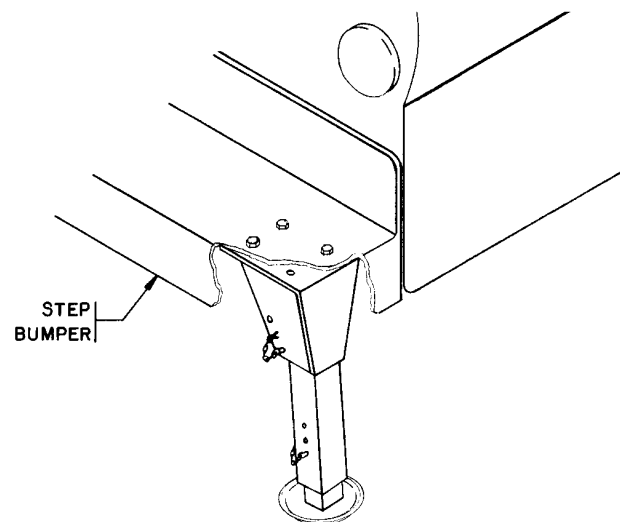
TYPICAL SHORT INSTALLATION OUTRIGGER
