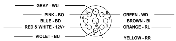
PLUG - BACKSIDE VIEW
