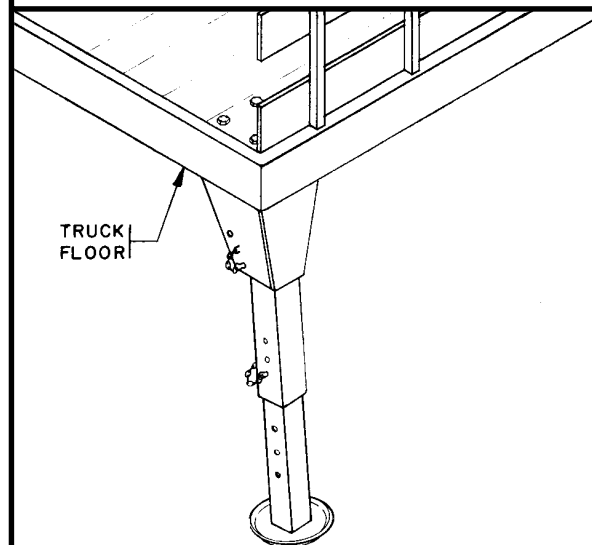
TYPICAL LONG INSTALLATION OUTRIGGER
