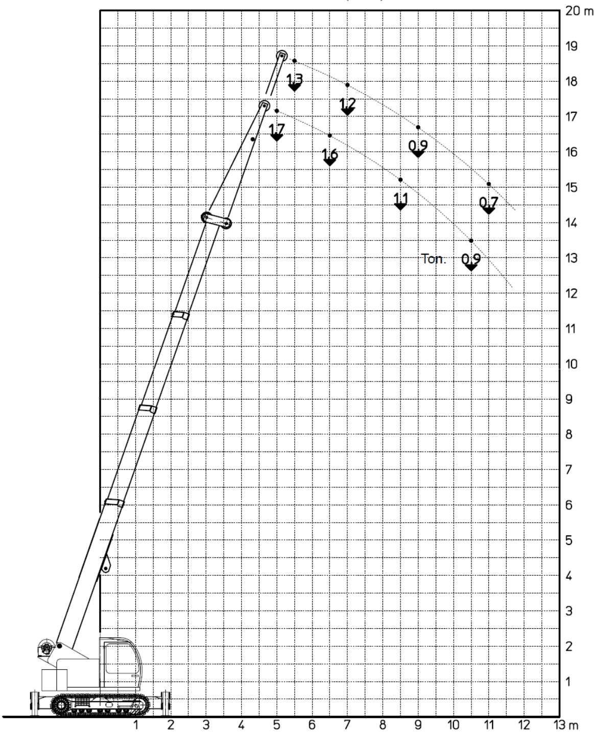
CAPACITY DIAGRAM FLY JIB ON OUTRIGGERS (360°)
