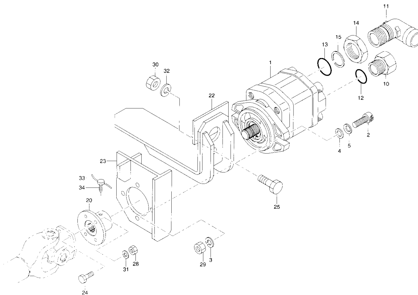
Fig. 25-5-2 PUMP FITTING ASS'Y(P.T.O. PROPELLER type)
