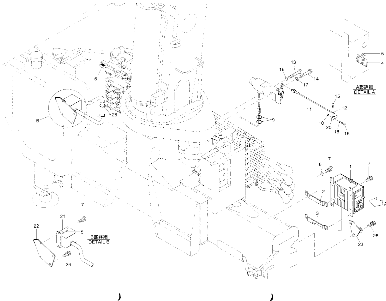
Fig. 21-1 リモコン取付配線組立(有線式) (URV370系 RK, R 仕様) REMOTE CONTROL FITTINGS & WIRINGS ASS'Y (Wired) (URV370 series RK & R type)
