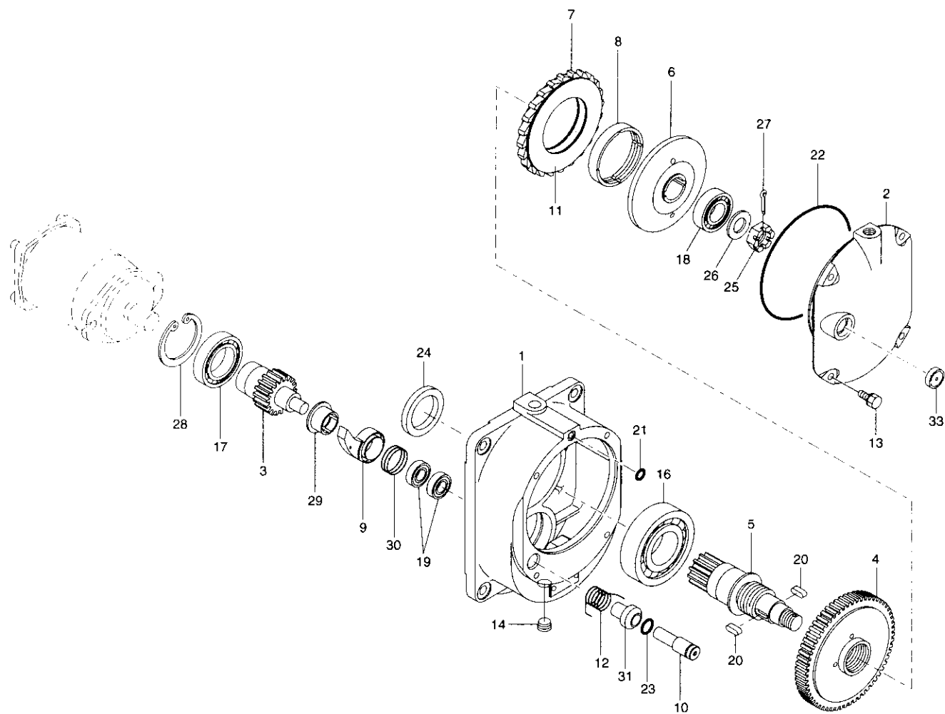
Fig. 10-1-1 HOIST WINCH REDUCTION GEAR ASS'Y (URV370 series K & STD type)
