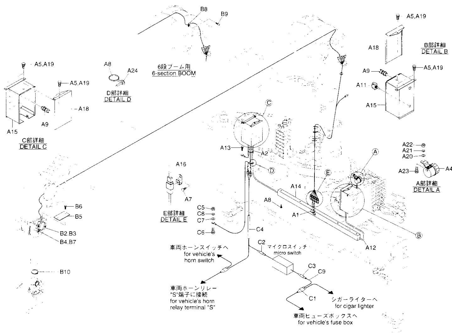
Fig. 4-2 ALARM DEVICE ASS'Y(URV370 series STD type)
