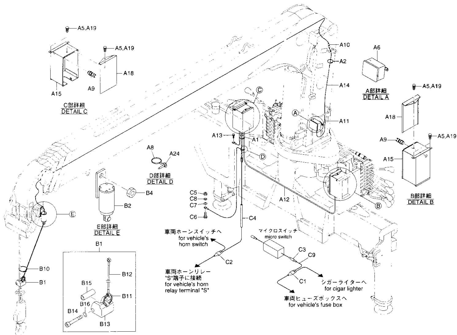
Fig. 4-4 ALARM DEVICE ASS'Y (URV370 series F type)
