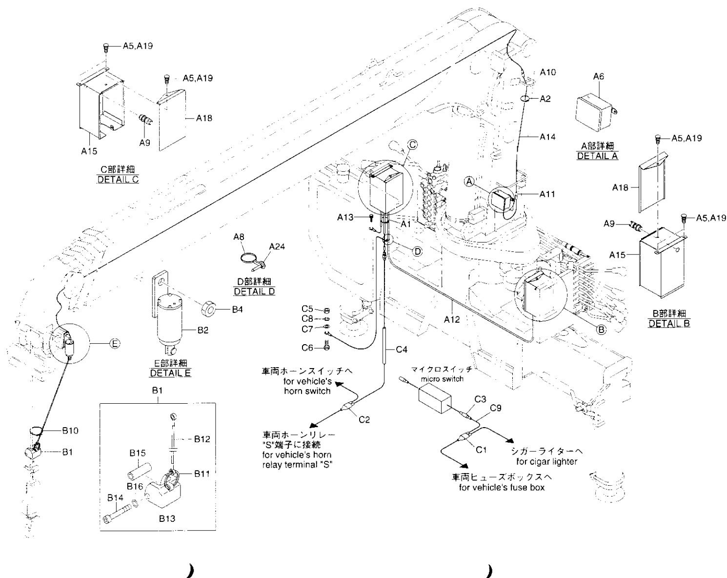
Fig. 4-4 ALARM DEVICE ASS'Y(URV370 series F type)
