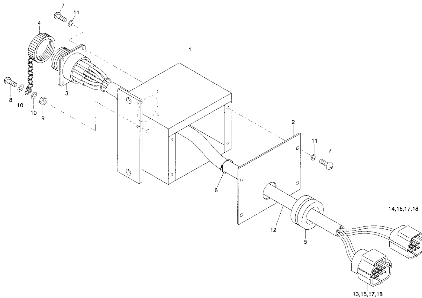
Fig. 21-1-2 CONNECTOR BOX ASS'Y (URV370 series RK & R type)
