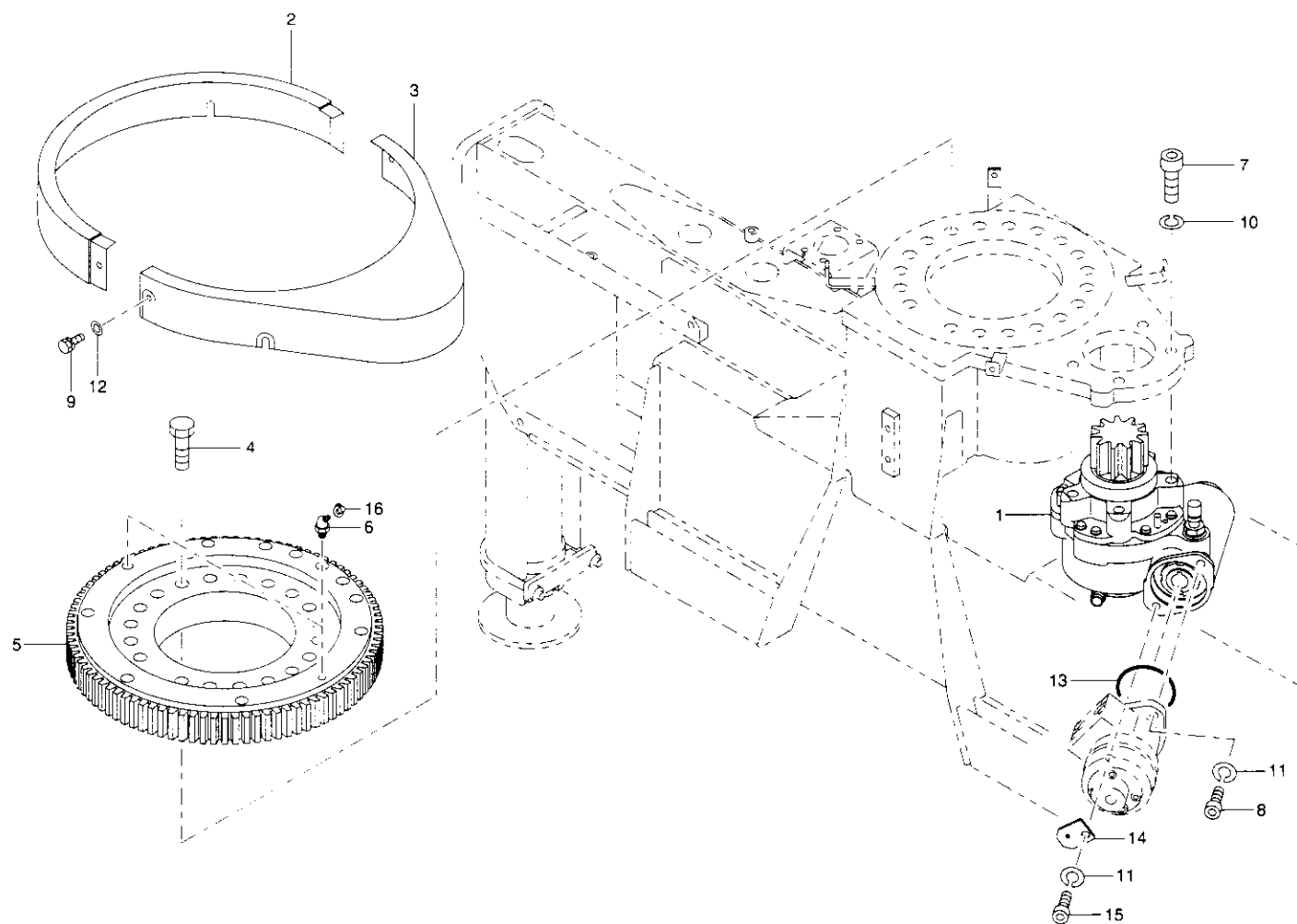
Fig. 9-1 SLEWING DEVICE ASS'Y(ALL MODELS)
