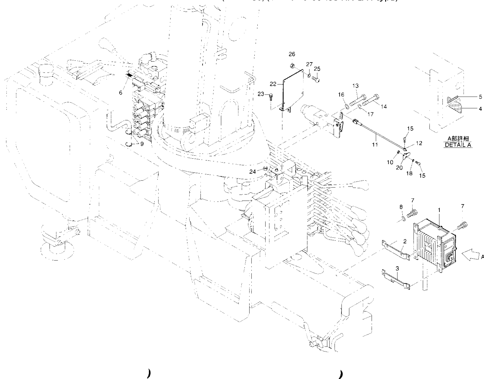
リモコン取付配線組立(無線式) (URV370系 RK, R 仕様) Fig. 21-2 REMOTE CONTROL FITTINGS & WIRINGS ASS'Y(Wireless) (URV370 series RK & R type)
