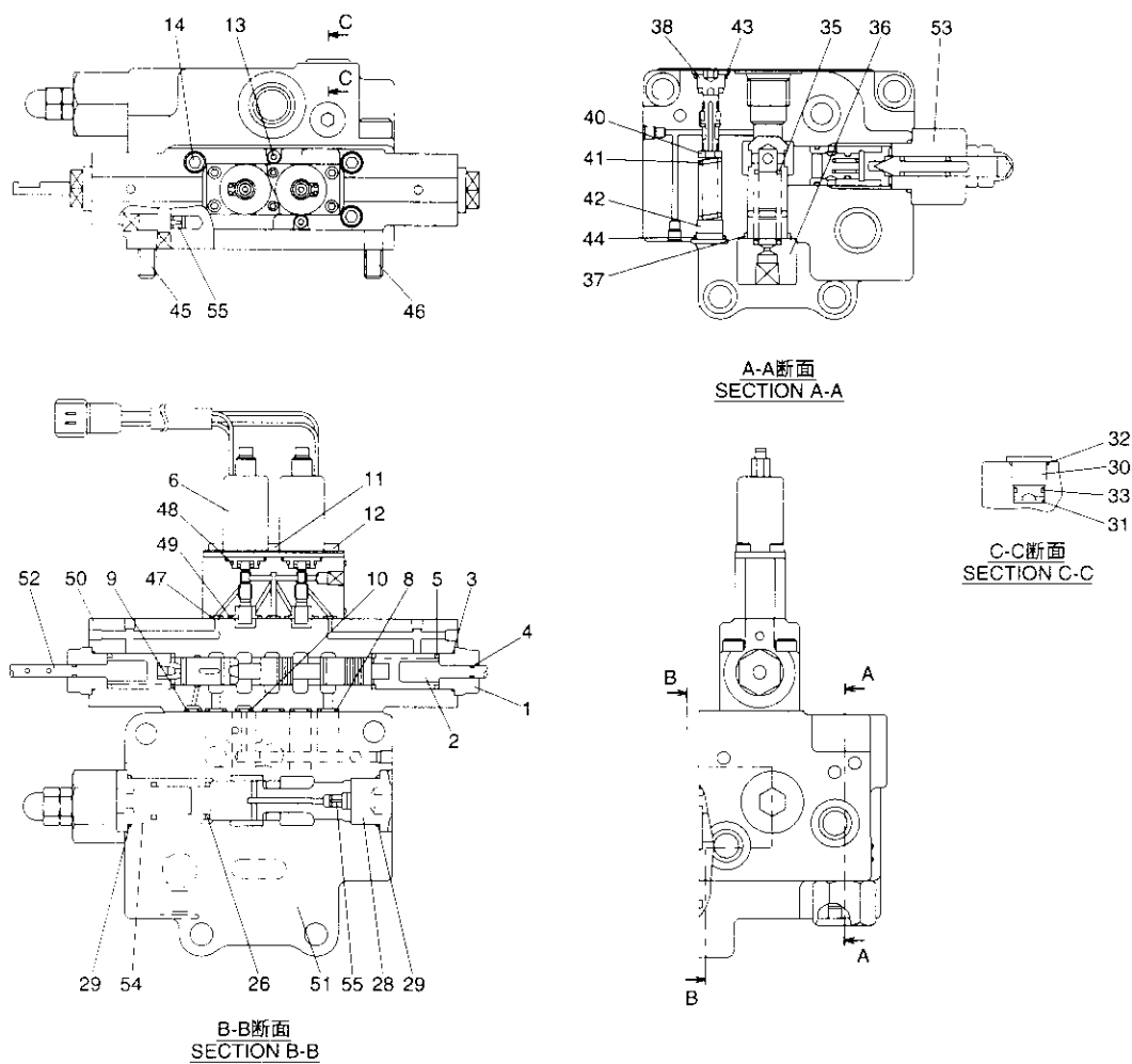
Fig. 24-3-1 吐出制御バルブASS'Y SOLENOID VALVE ASS'Y
