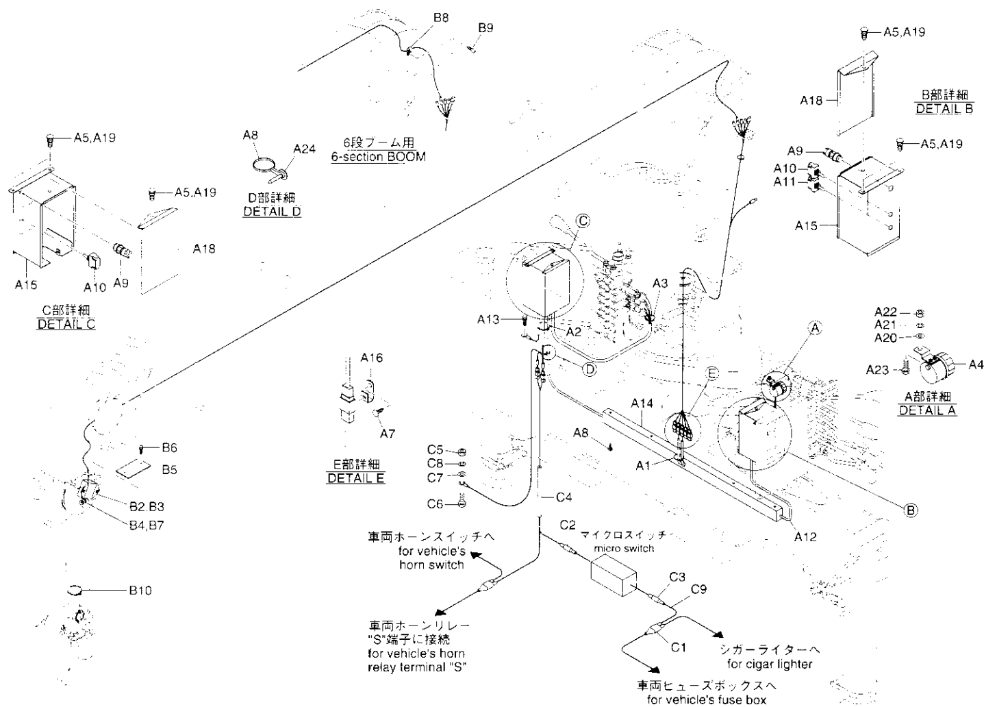
Fig. 4-1 ALARM DEVICE ASS'Y(URV370 series K type)
