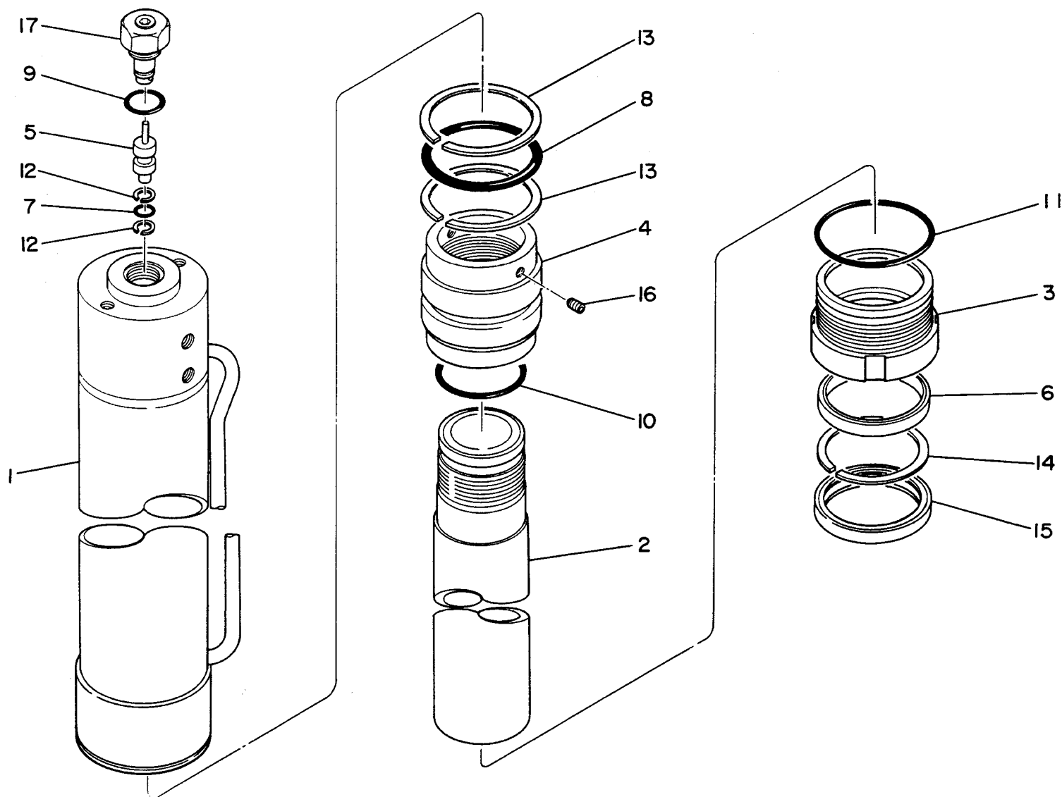
Fig. 16 OUTRIGGER CYLINDER ASS'Y
