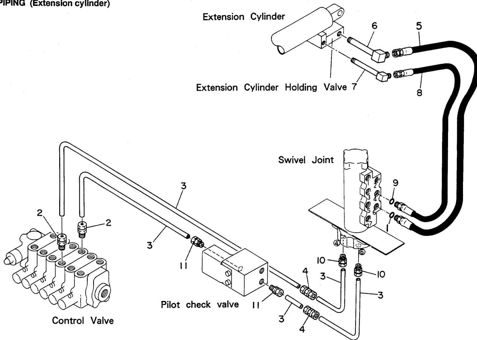
Fig. 8-3 PIPING (Extension cylinder)
