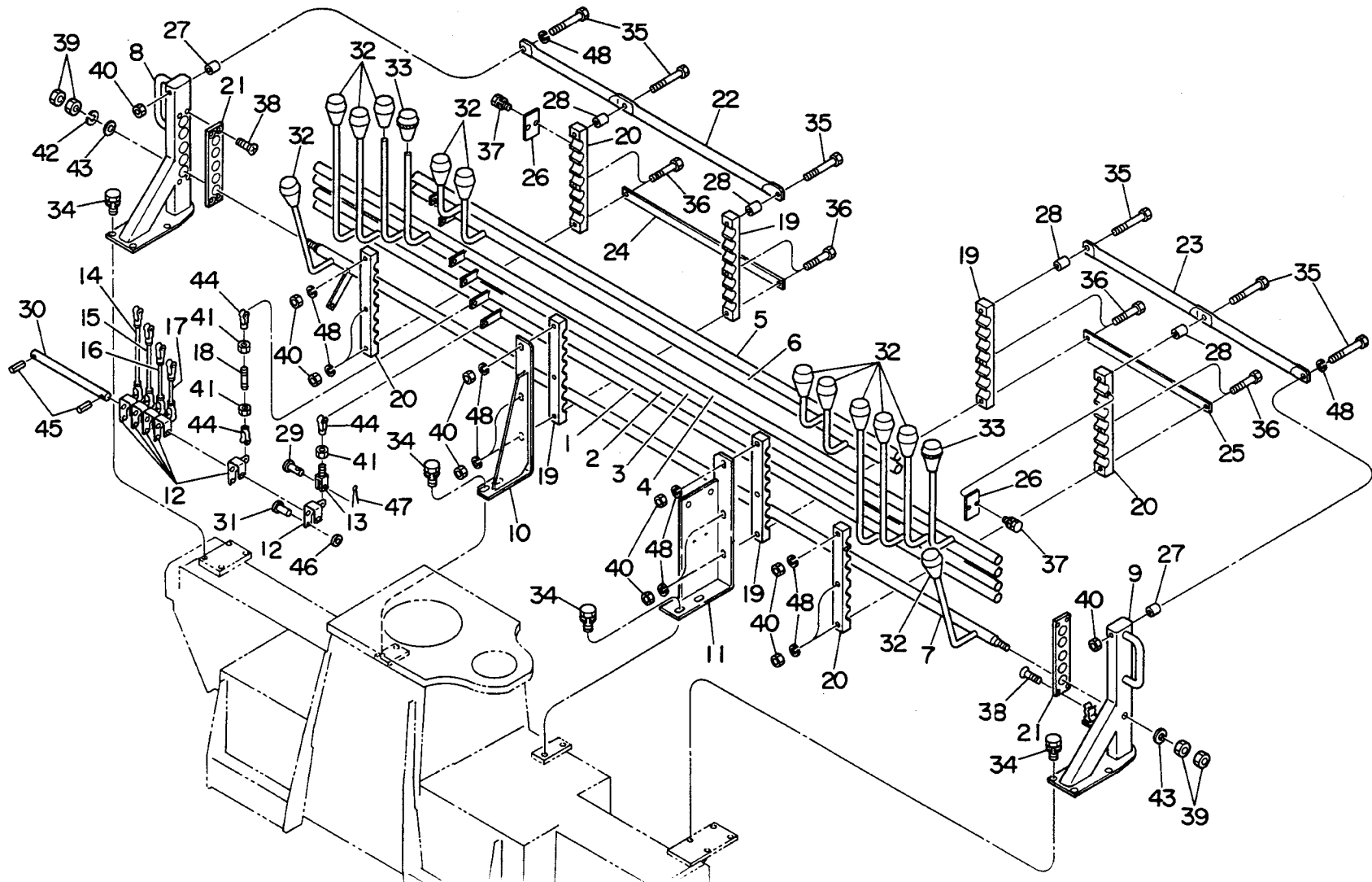
Fig. 19 CONTROL ASS'Y
