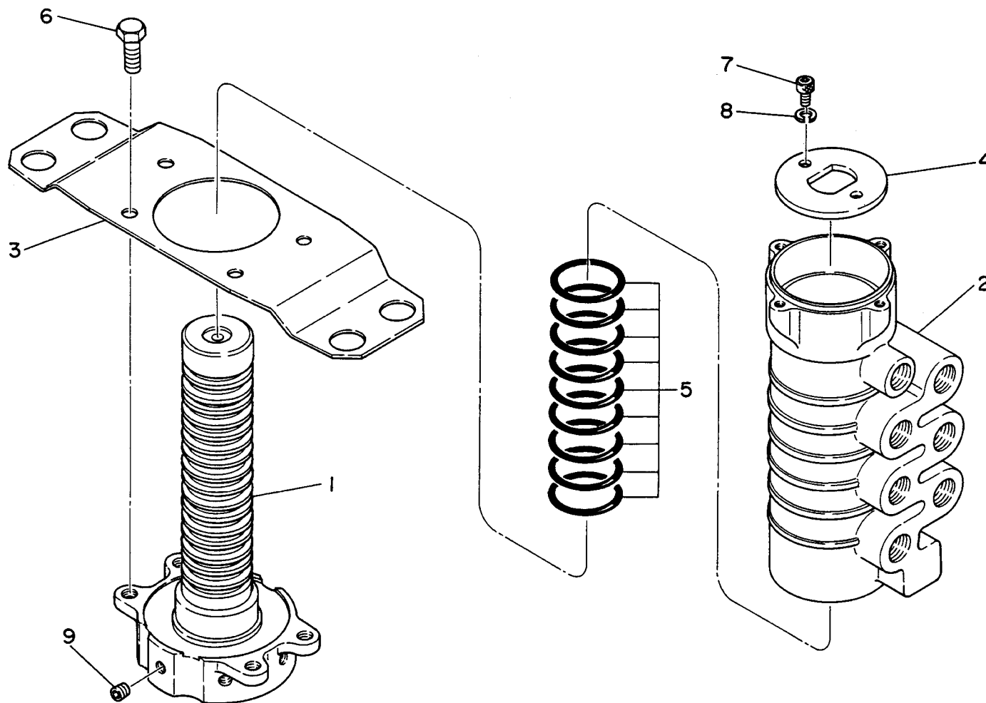
Fig. 17 SWIVEL JOINT ASS'Y
