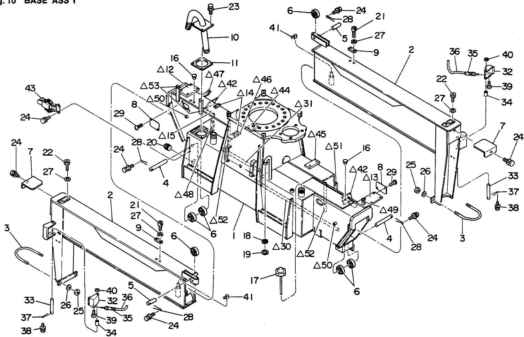
Fig. 10 BASE ASS'Y
