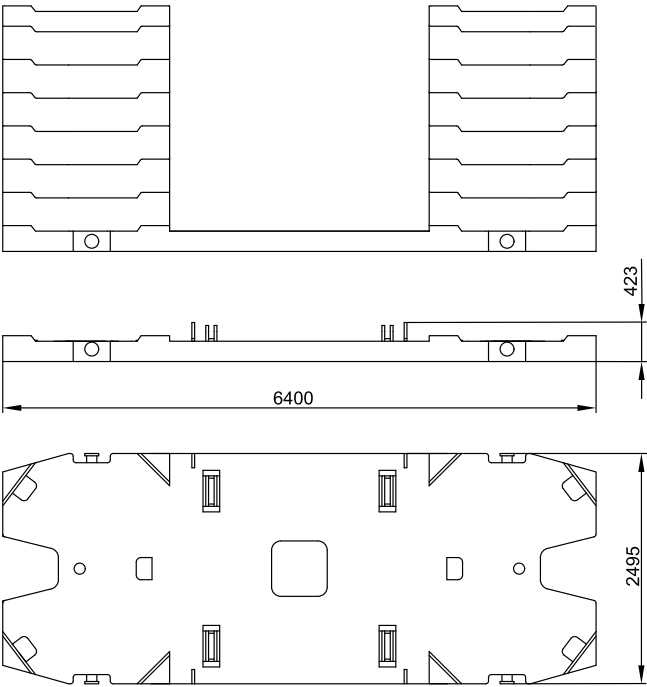
Counterweights on upper · 上车配重
