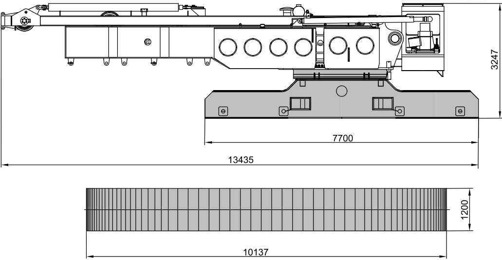
Counterweights on upper · 上车配重
