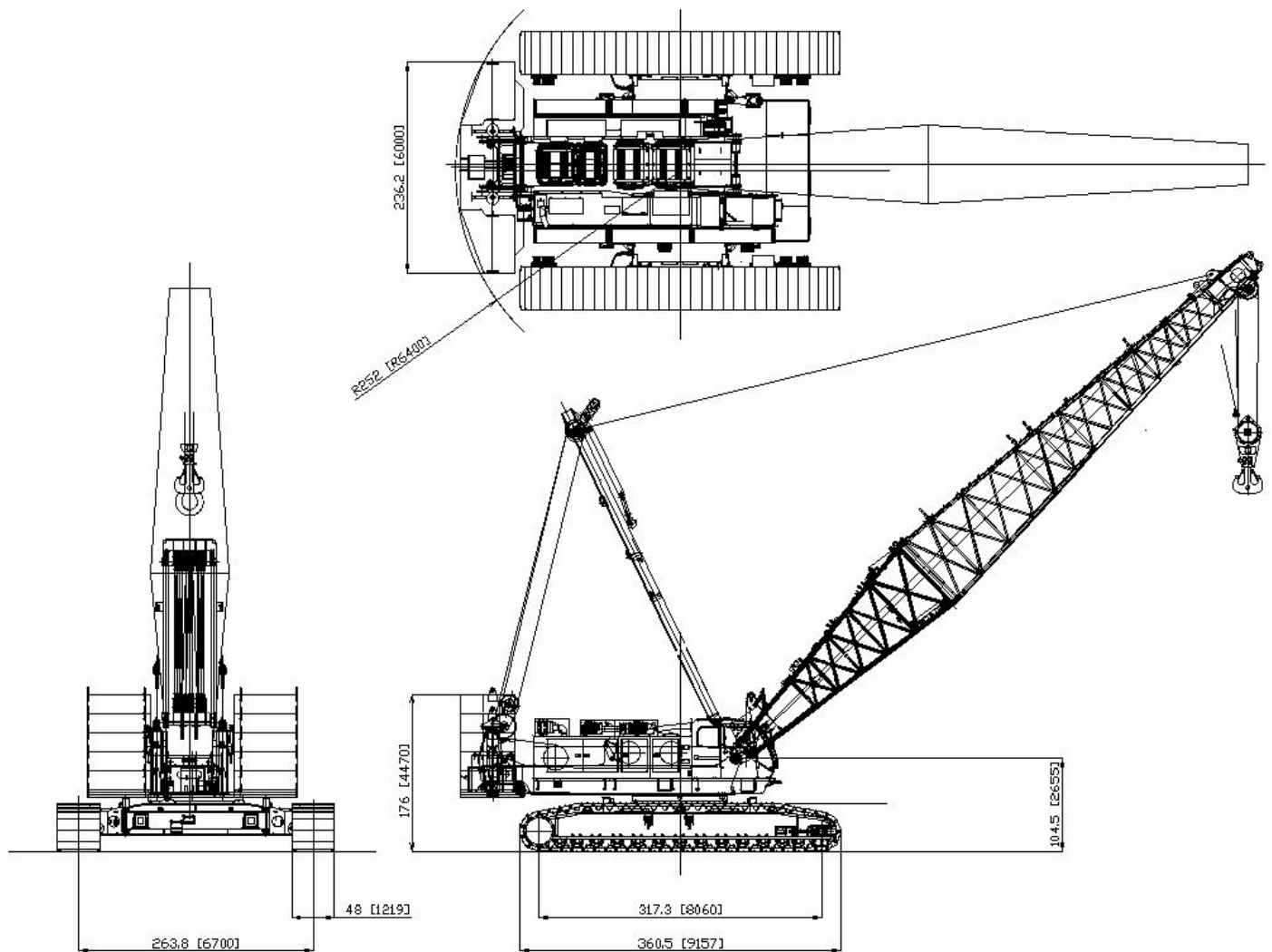
HC285 BASIC MACHINE
