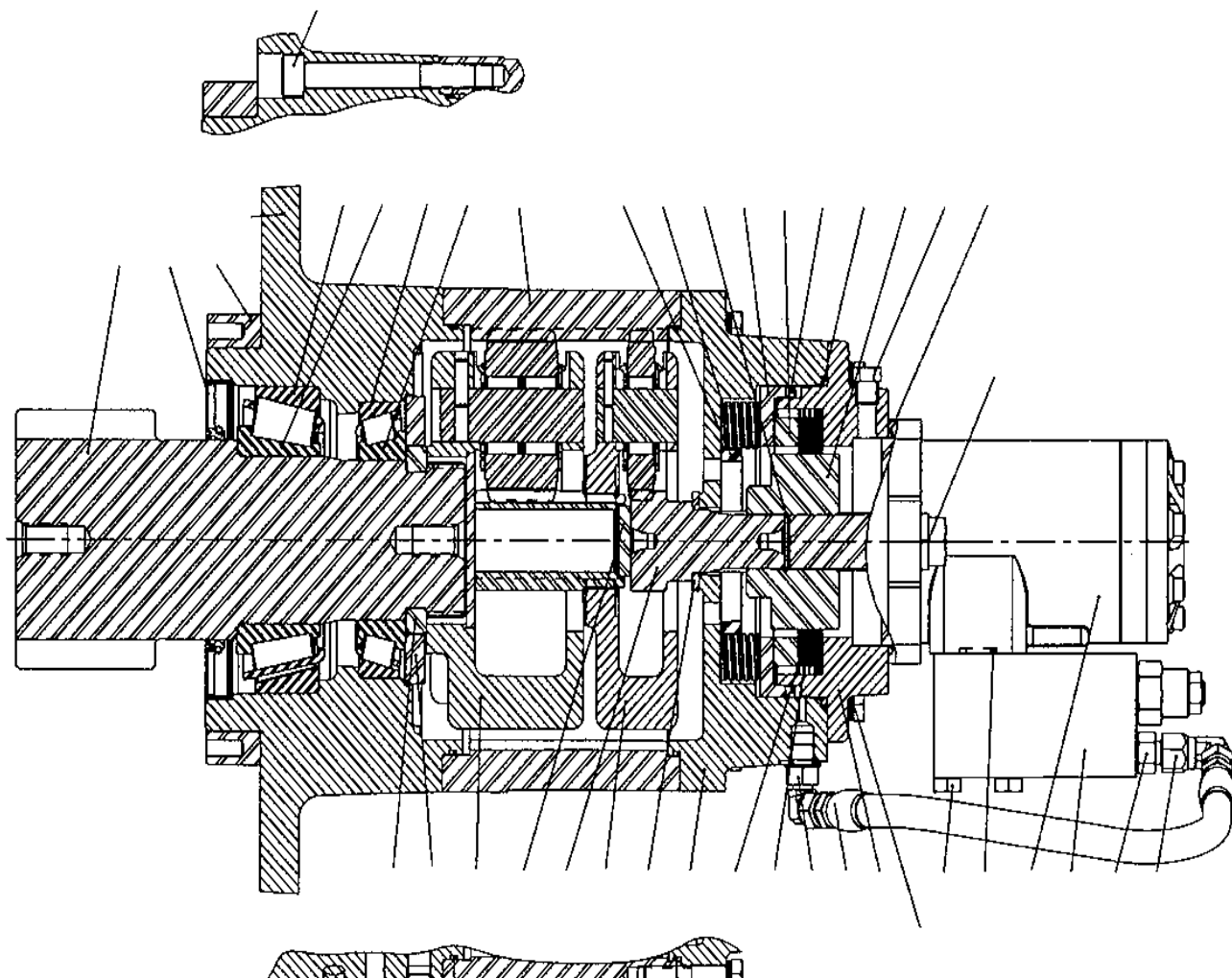
Rotation Gearbox Assembly
