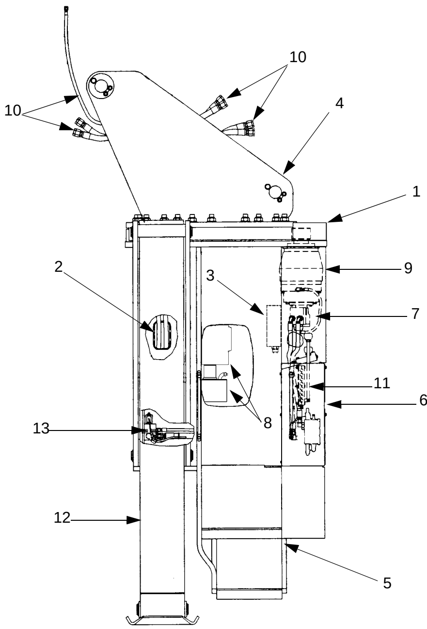
Mainframe Assembly, Continuous Rotation
