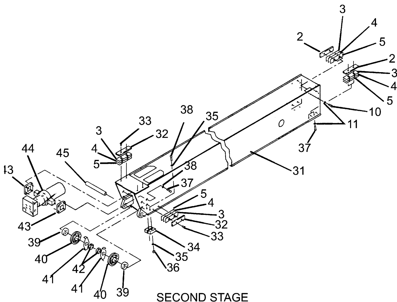
SECOND STAGE Boom Assembly - 57' 2nd Stage
