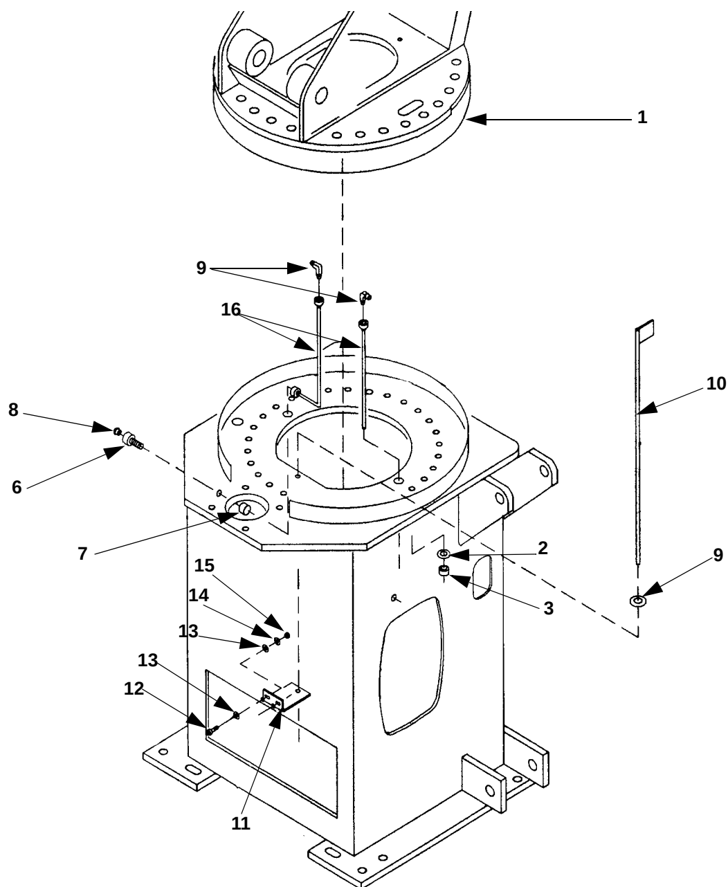
370 Deg Rotation Stop Installation
