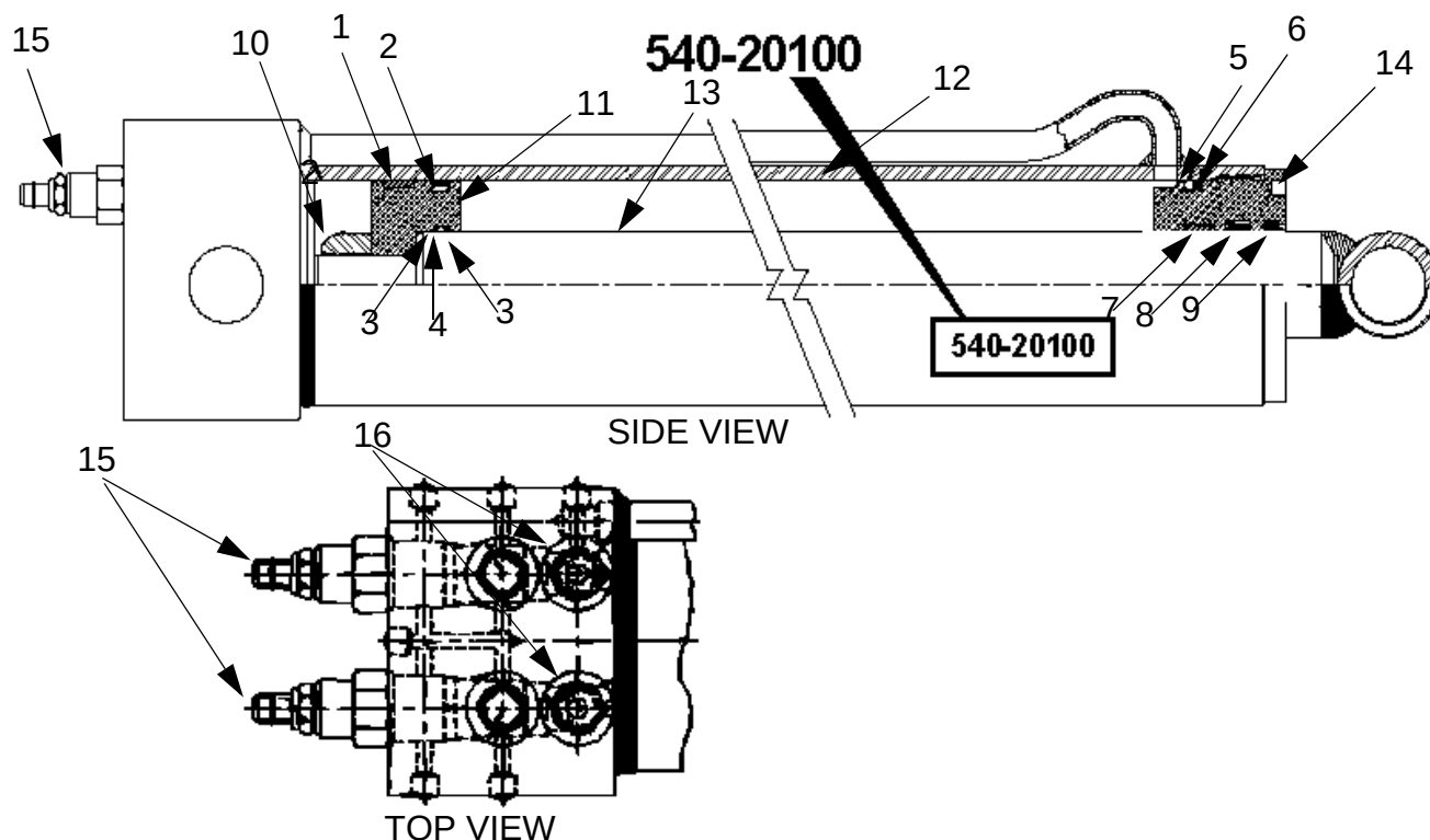
Auxiliary Outrigger Cylinder
