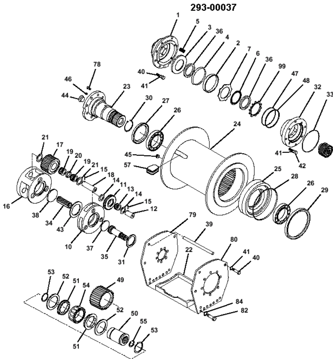
Winch Assembly
