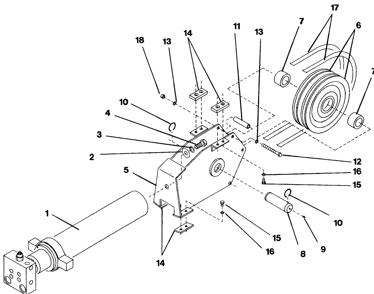
Extension Cylinder Assembly 57'
