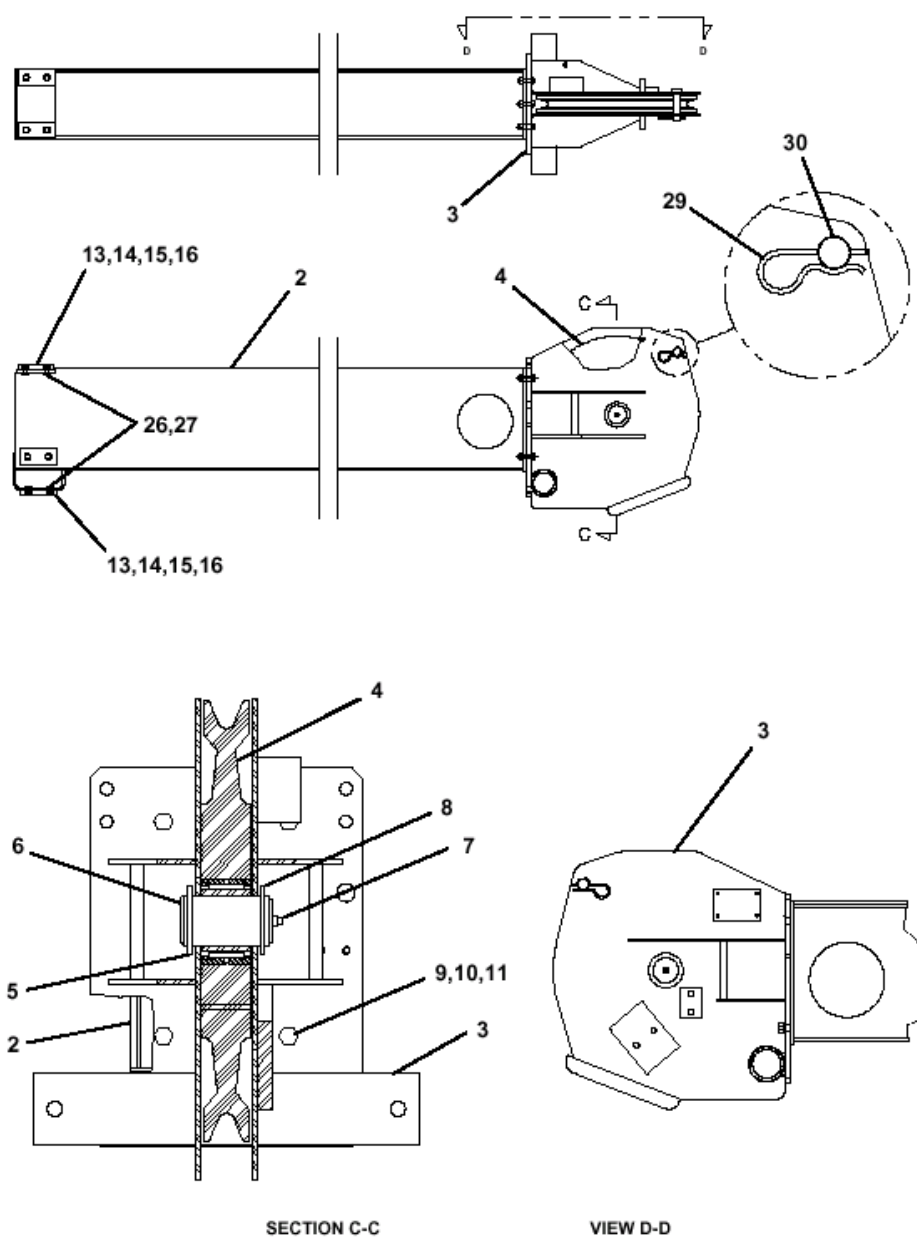
2 Stage JIB Assembly 92'
