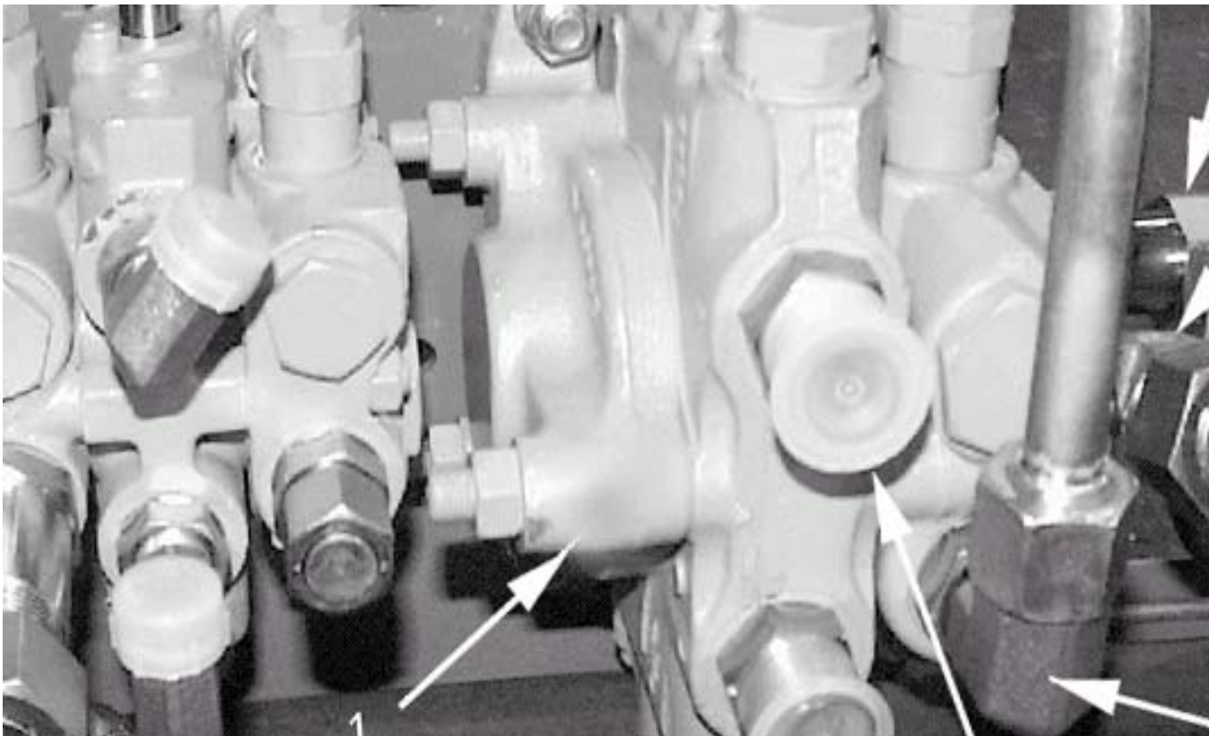
Winch Valve Assembly-Husco
