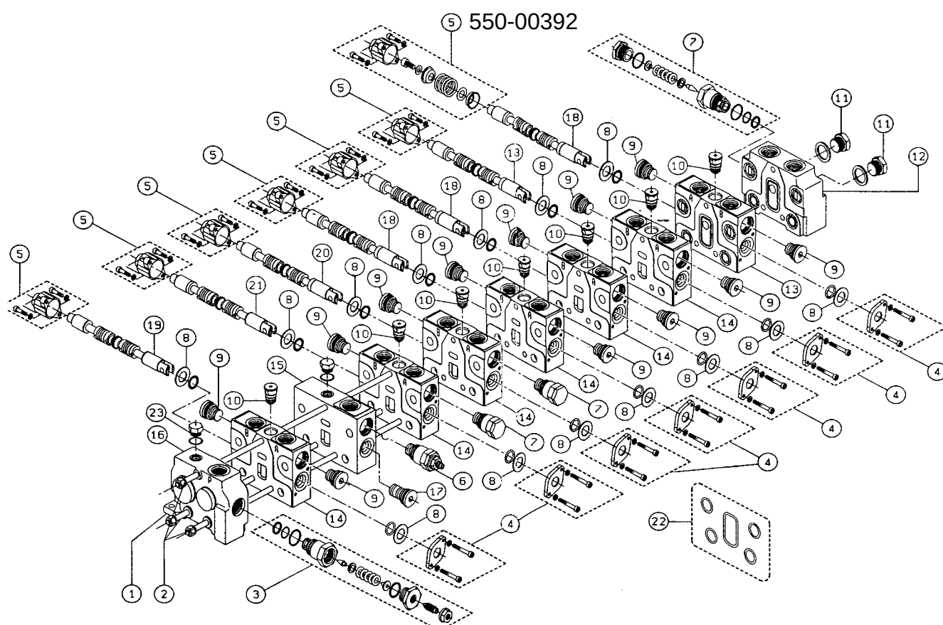
Exploded View Main Valve Assembly-Salami
