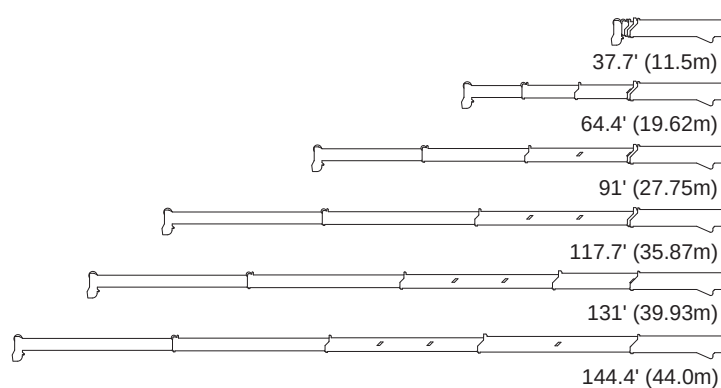
Boom Length in Feet (Telescoping Mode II)
