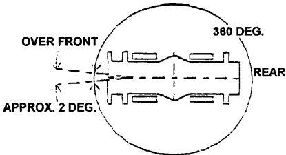
WORKING AREA DIAGRAM WITHOUT OUTRIGGERS 'OVER FRONT' OPERATION SHOULD BE PERFORMED WITHIN 2 DEGREES IN FRONT OF CHASSIS.
