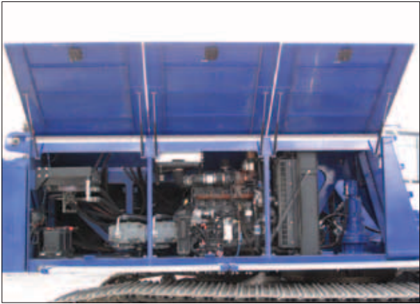
Large access doors, spacious machinery compartments simplify preventative maintenance and service of the crane.
