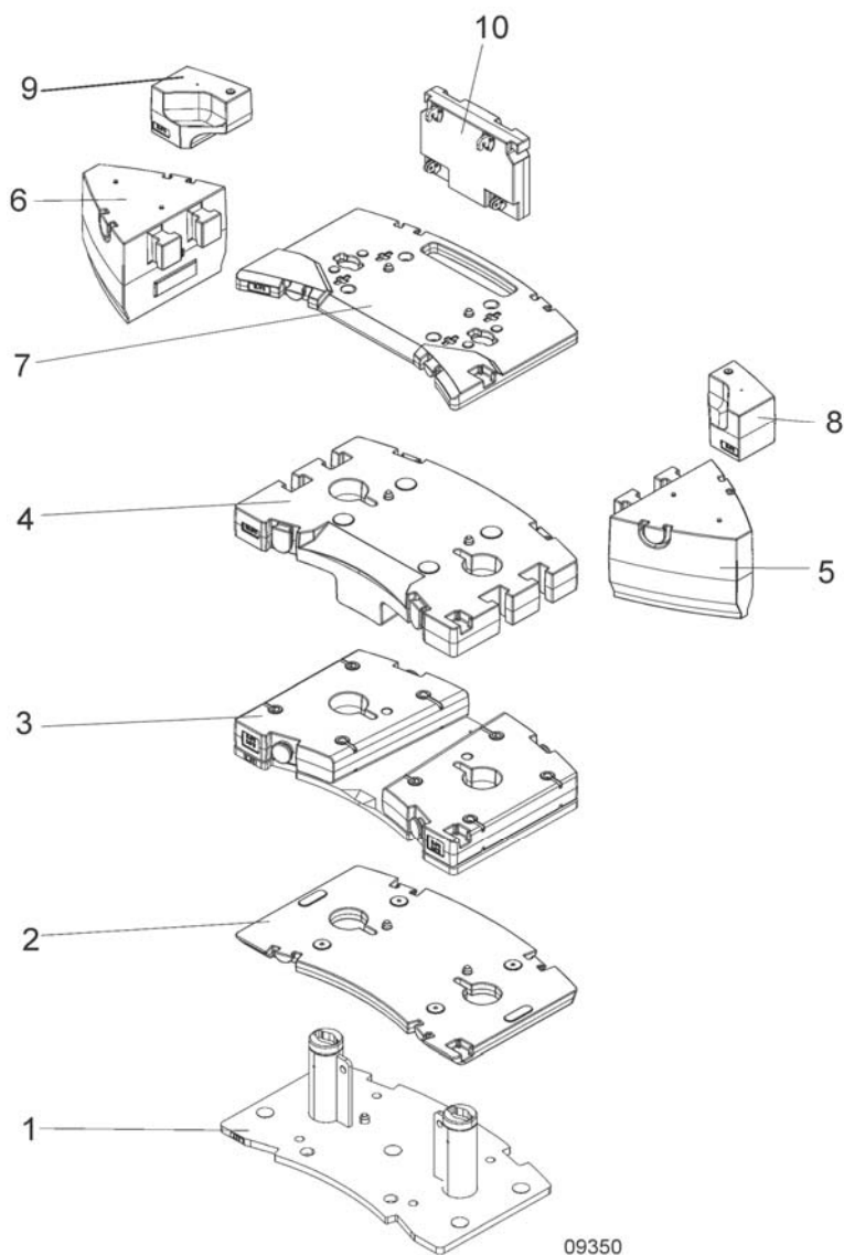
Mounting the 92,593 lbs (42 t) counterweight
