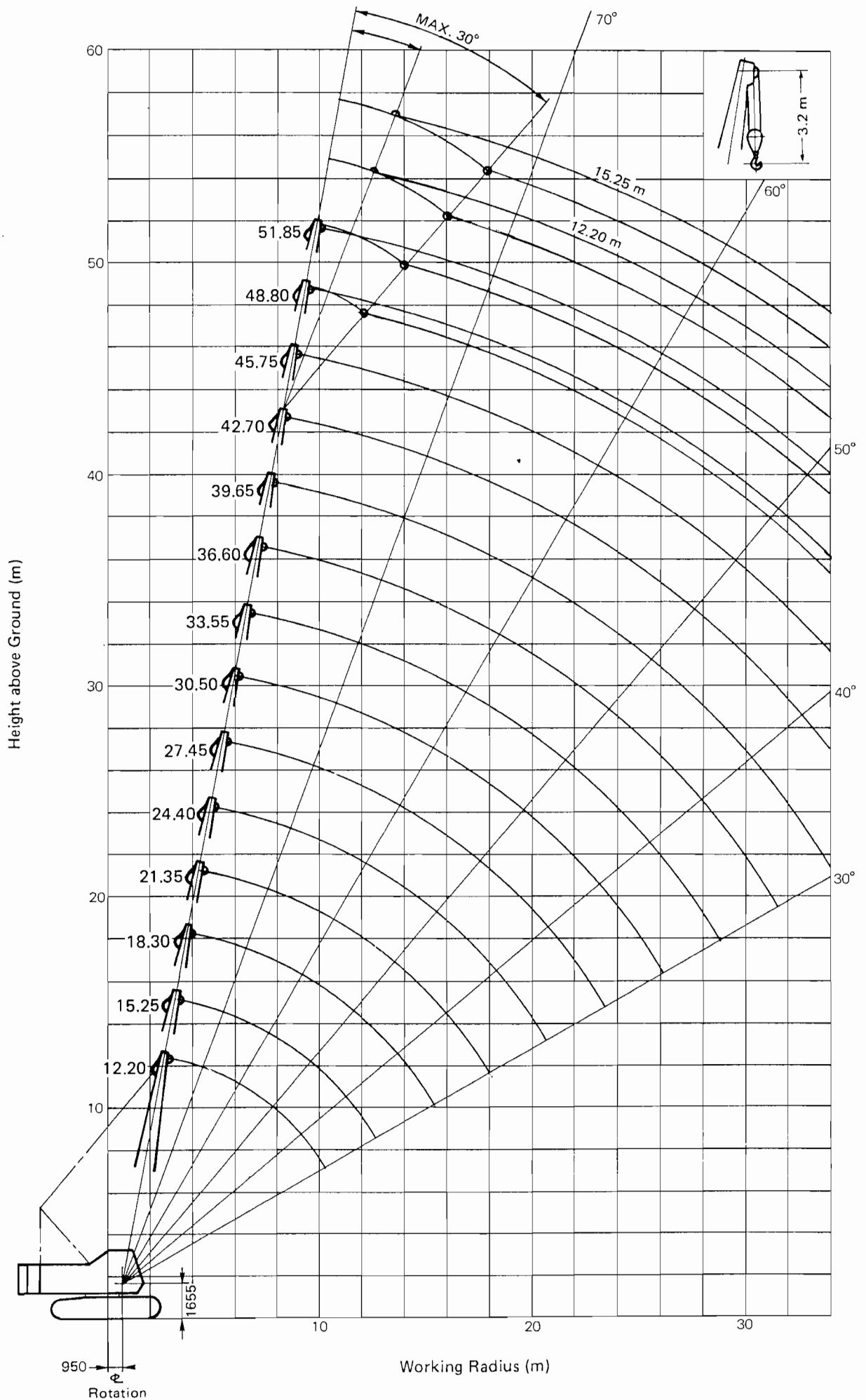
LS-118RH-5 CRANE WORKING RANGES
