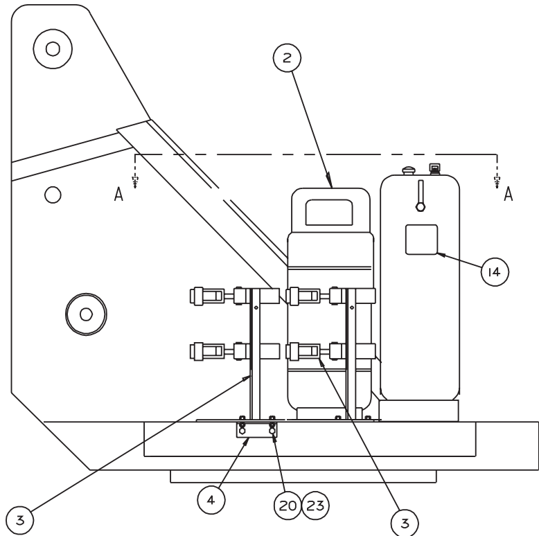
TURNABLE-R.H.SIDE
