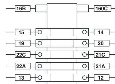
VICKERS PACKAGE VALVE WIRING
