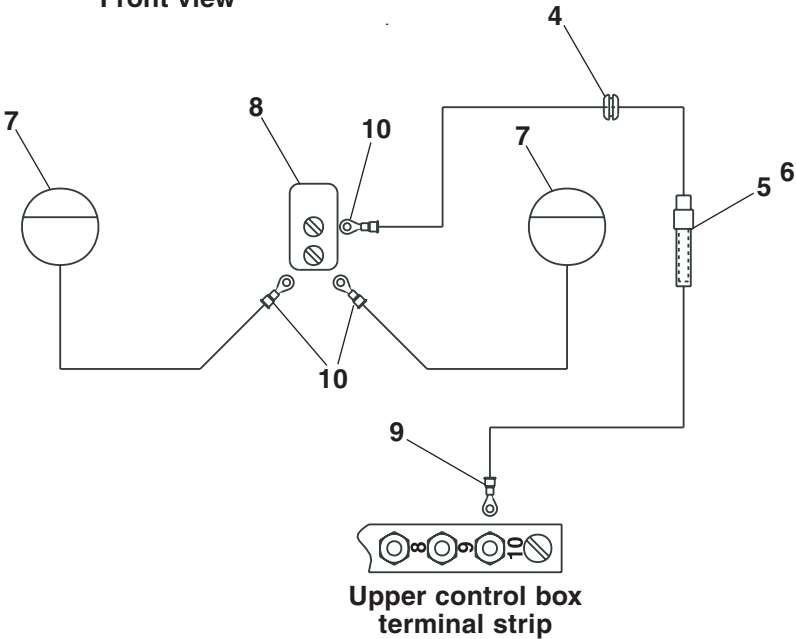
Upper control box Front view
