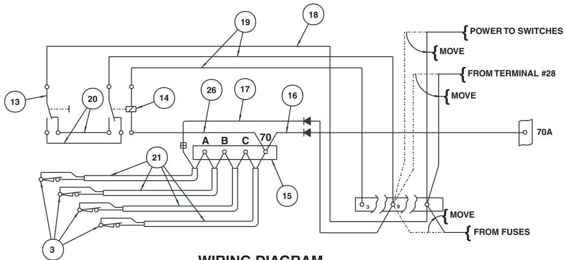
WIRING DIAGRAM
