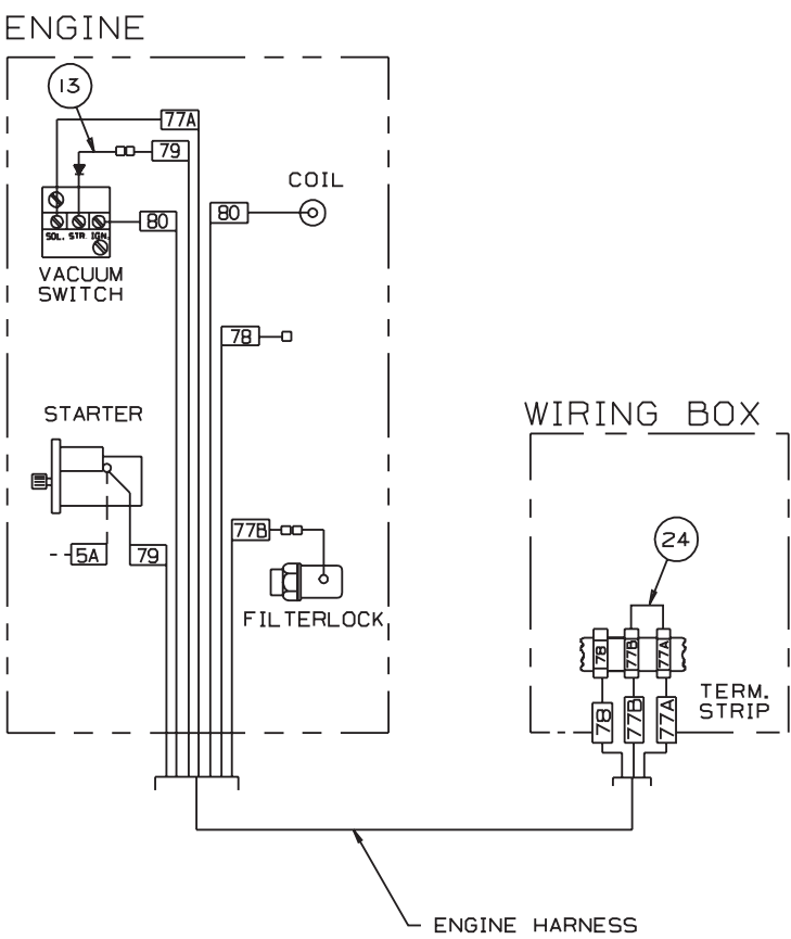
ENGINE HARNESS
