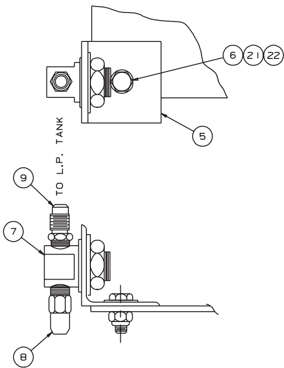
VIEW B-B
