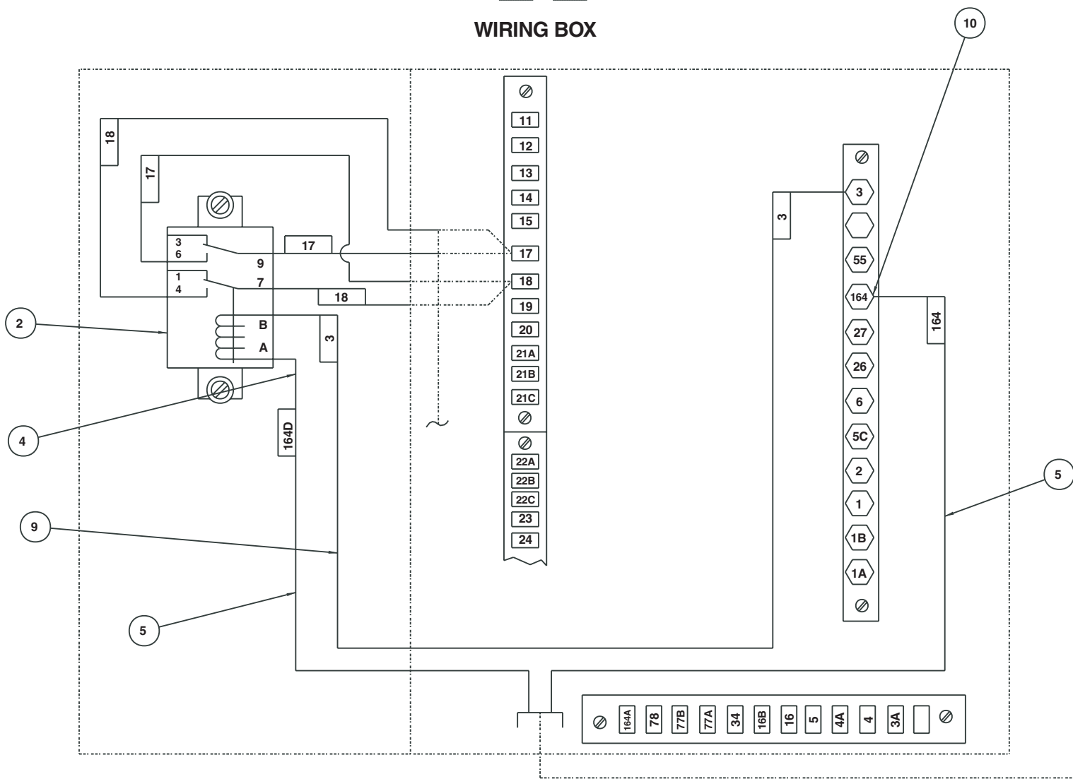
ELECTRICAL SCHEMATIC
