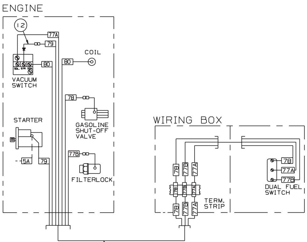
ENGINE HARNESS
