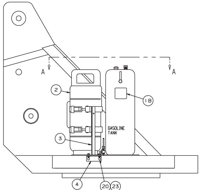
TURNABLE-R.H.SIDE
