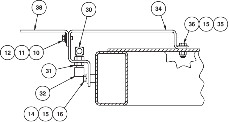
VIEW B-B
