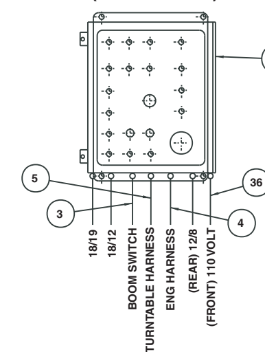
WIRING BOX (FRONT VIEW)
