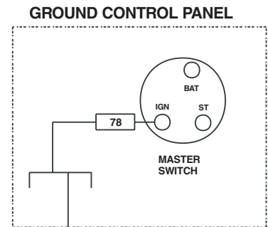
ENGINE WIRE ASSEMBLY (FO)
