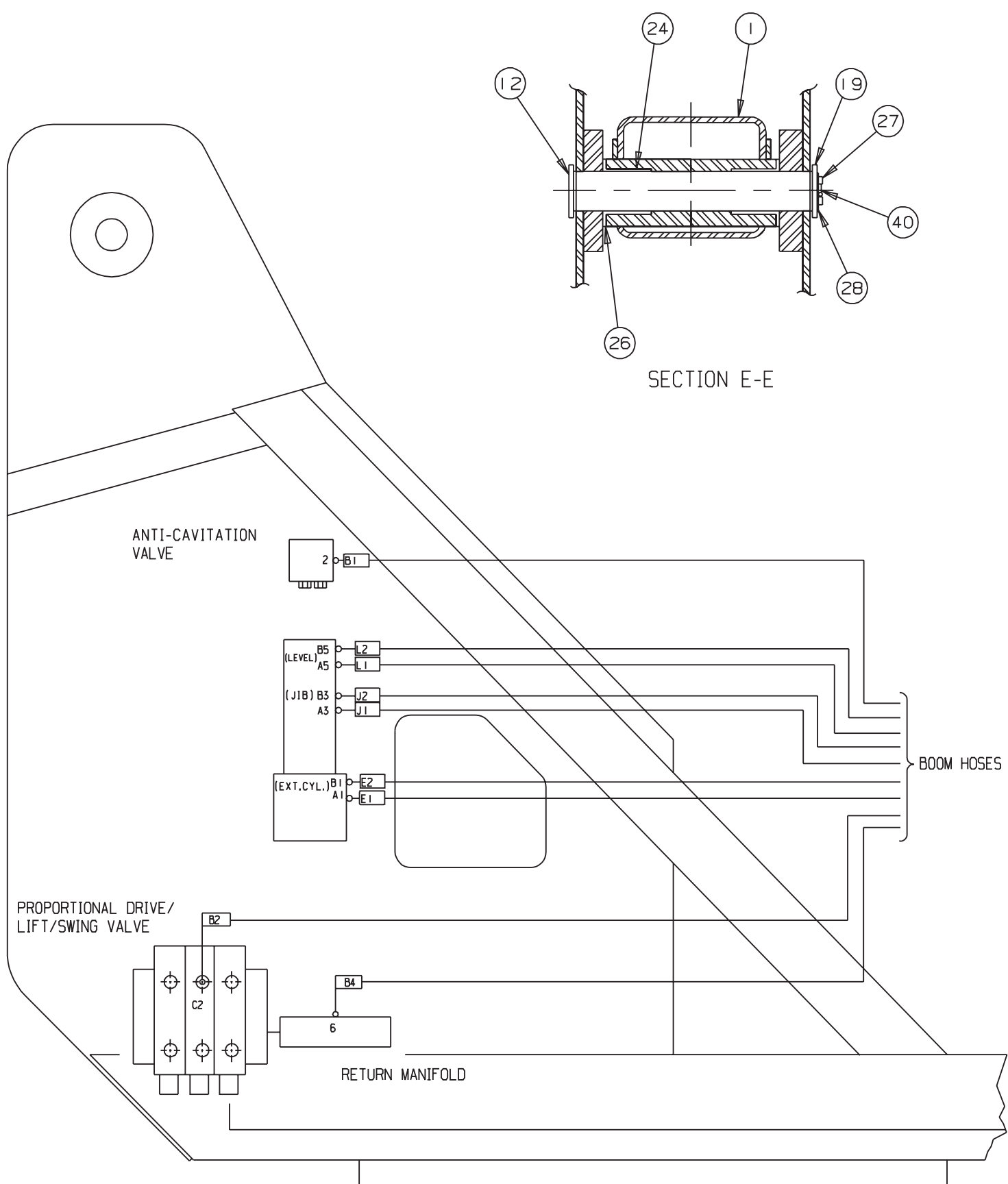
VIEW D-D
