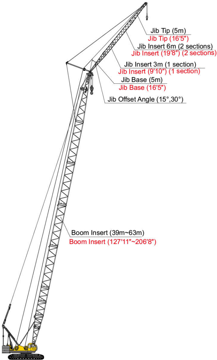
Combination of Jib 13m(42' 8" ), 19m(62' 4" ), 25m(82' )
