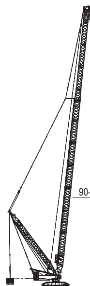
HJDB operating condition of mixed boom with superlift
