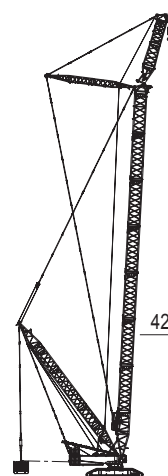
SF L DB operating condition of light-duty fixed short jib with superlift
