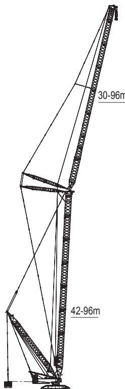
LJDB operating condition of luffing jib with superlift
