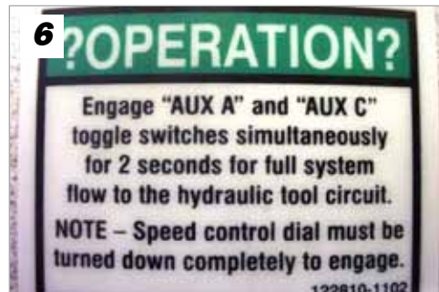
Toggle switches on the remote can be activated in dual operation mode by following the instructions on this decal
