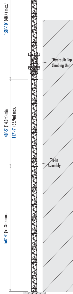
TOP CLIMBING with S35 Tower Sections (Tied to Structure)
