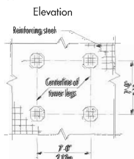
FOUNDATION DETAILS (Concrete Slab)
