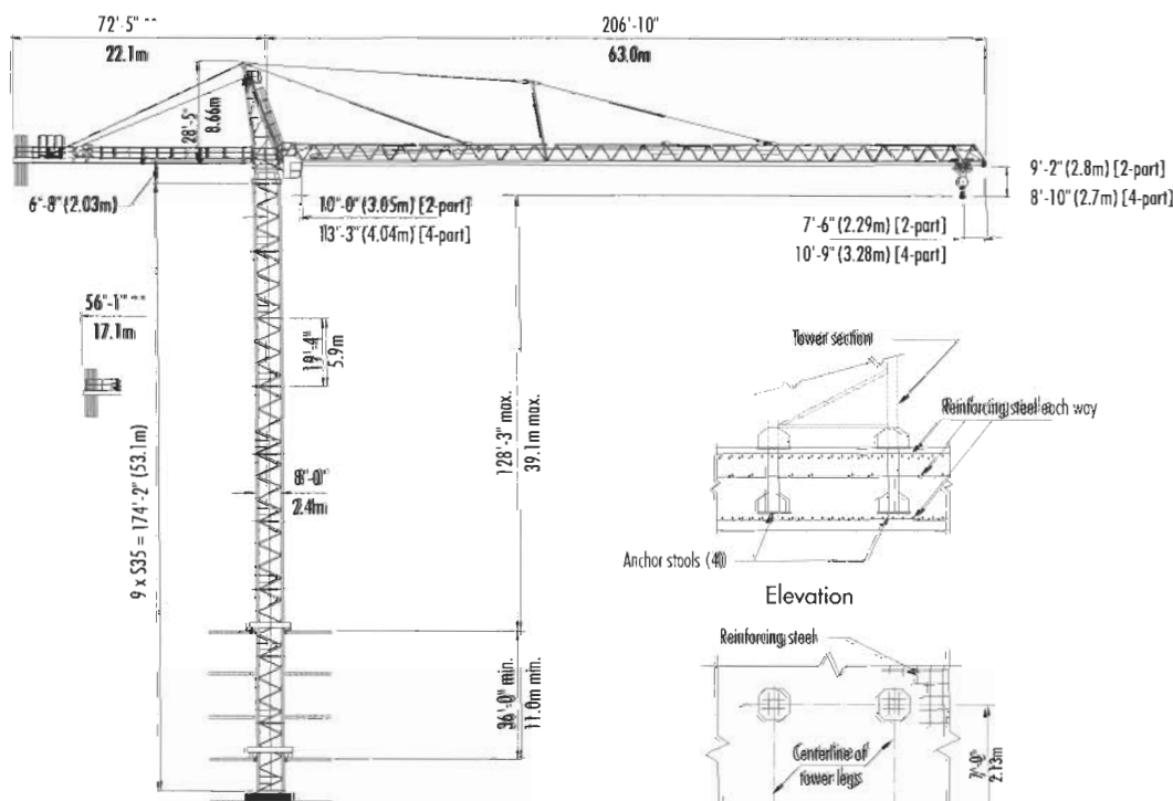
BOTTOM CLIMBING with S35 Tower Sections (Inside Structure)
