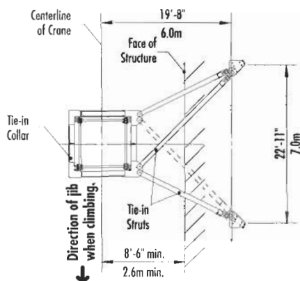
TIE-IN ASSEMBLY (Plan View)
