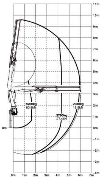
PK 12502 Performance
