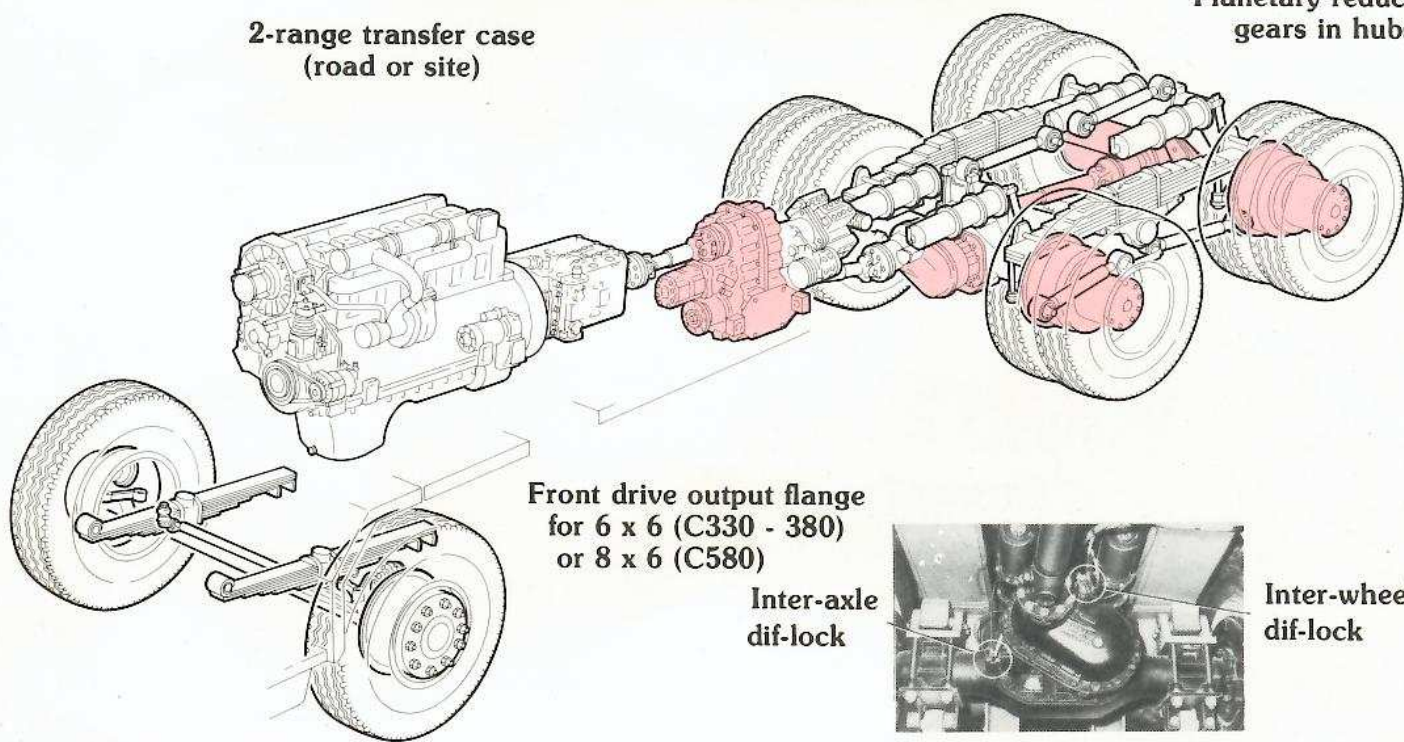
Optional front drive axle
