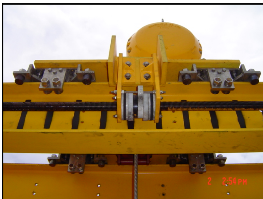
Figure 8 - Stainless Steel Rollers and Acme Drives
