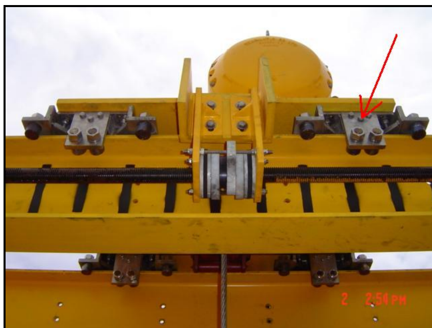
Figure 21 - Winch Trolley Lower Rollers
