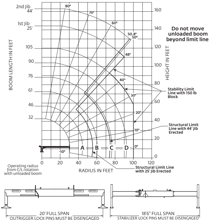
Load chart
