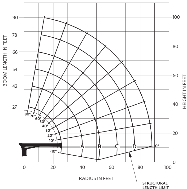
Load chart
