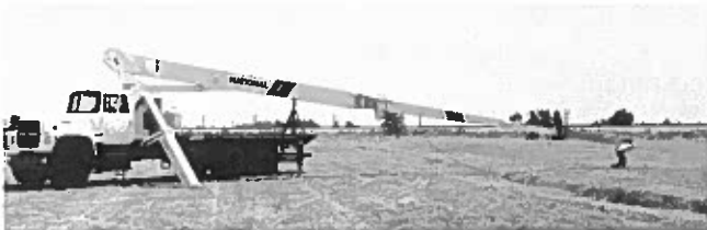
This photo sequence demonstrates how a National jib folds out into working position.
