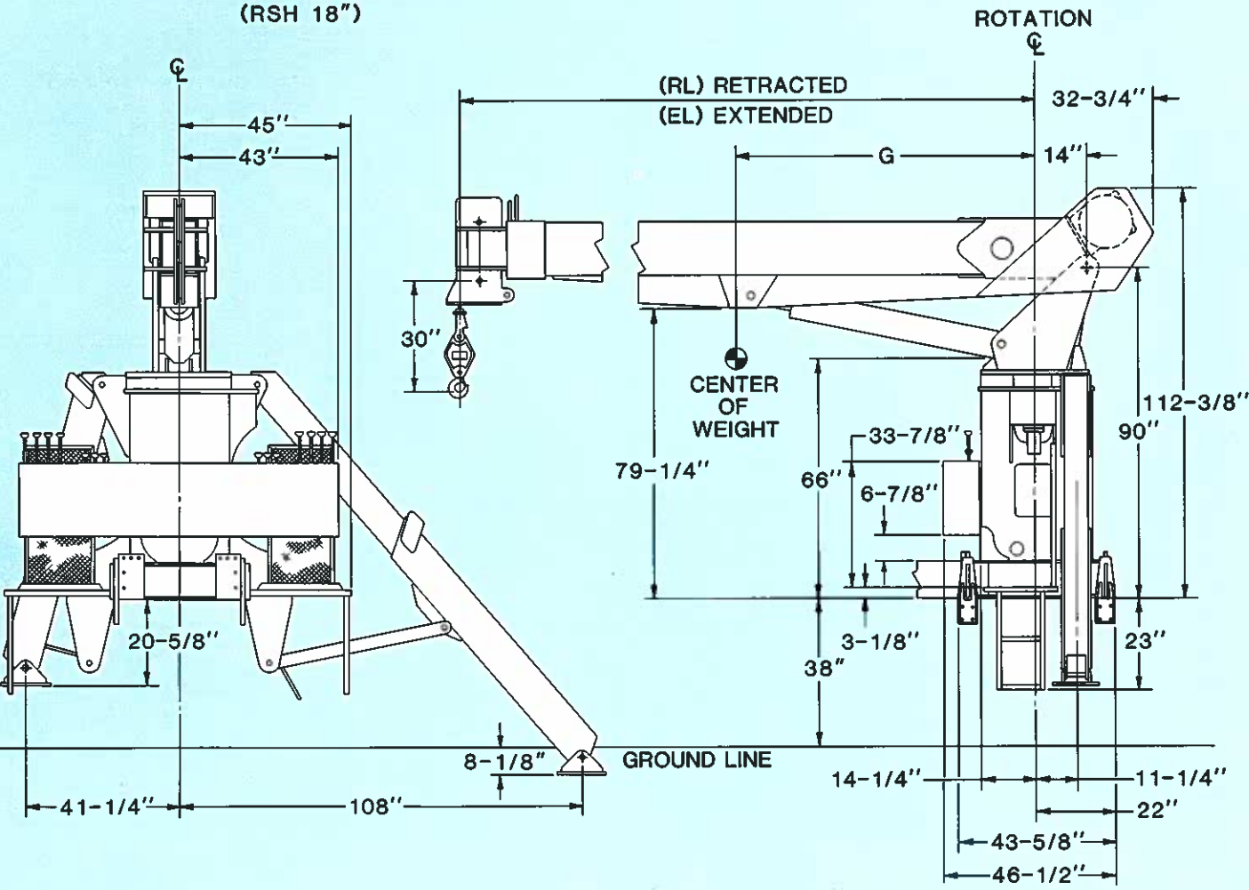
REAR STABILIZER (RSH 18")
