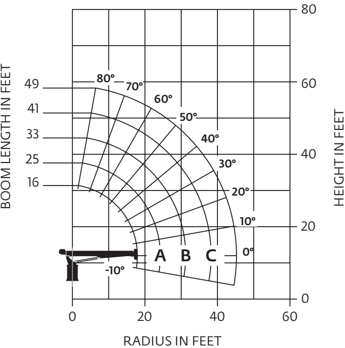
Load chart
