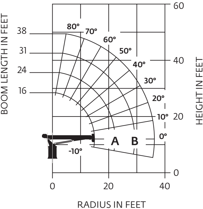
Load chart
