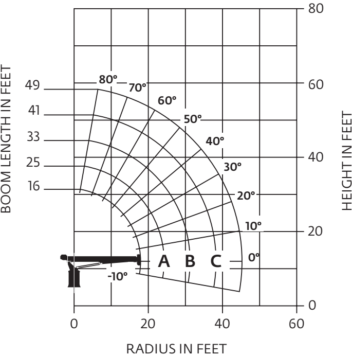
Load chart
