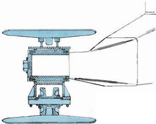
SECTION SHOWING METHOD OF ATTACHING CARBODY AXLE ENDS TO CRAWLER FRAME
