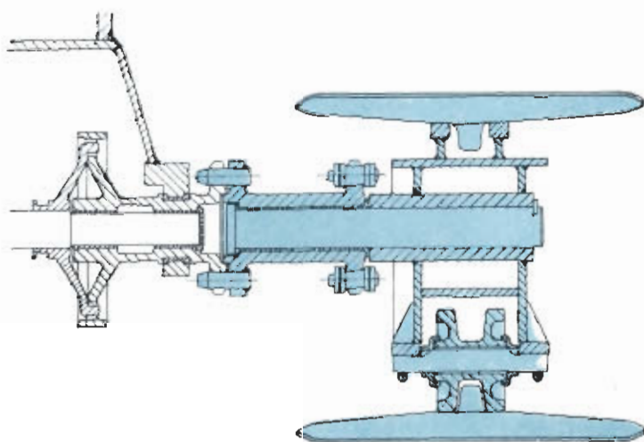
SECTION SHOWING DRIVE FROM LOWER TRACTION SHAFT
