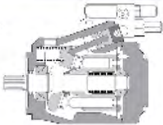
The axial piston pump with Load-Sensing control ensures a rapid response to all operator requirements.
