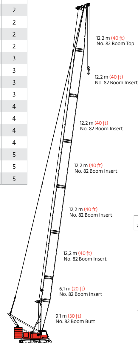
Model 999 Series 3 No. 82 or 22EL Boom 88,4 m (290 ft)
