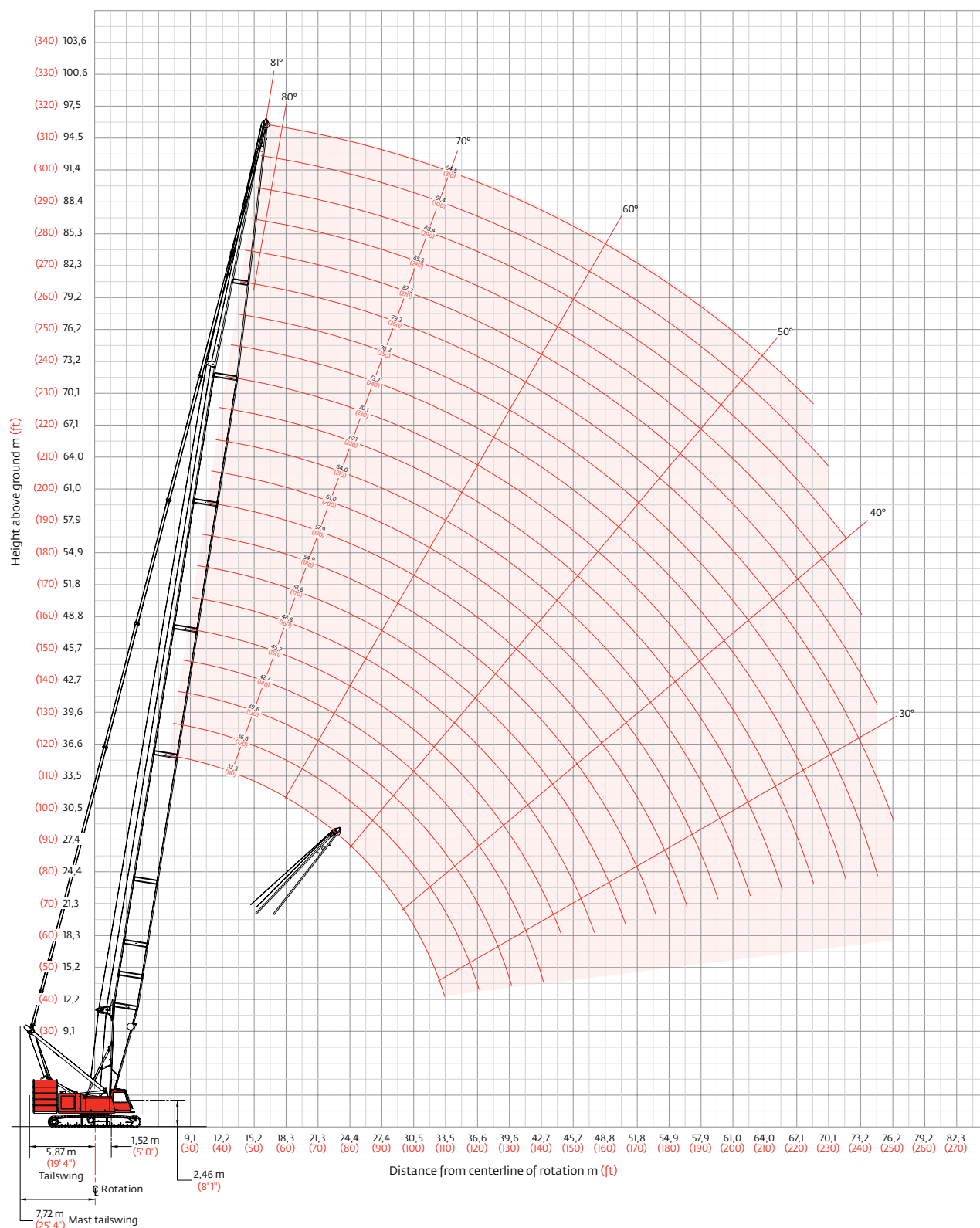
No. 22E Main boom with light tapered top
