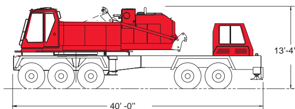
APPROXIMATE GROSS WEIGHT: 100,240 LB
