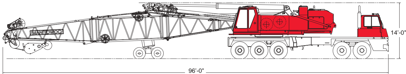
APPROXIMATE GROSS WEIGHT: 137,925 LB
