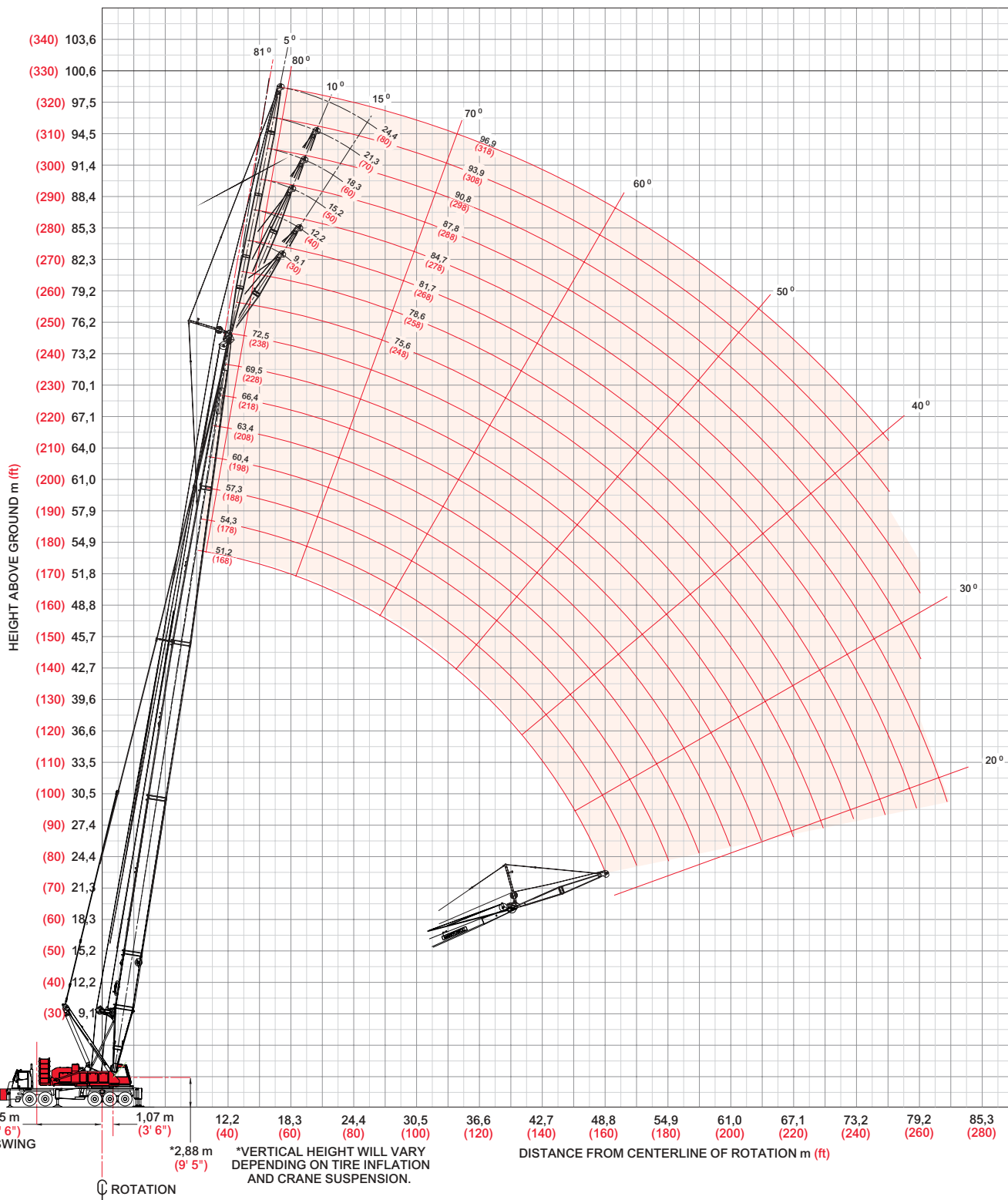
No. 138 Fixed Jib on Boom No. 78T with Long Reach Top
