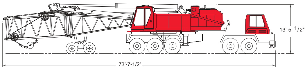
APPROXIMATE GROSS WEIGHT: 127,385 LB
