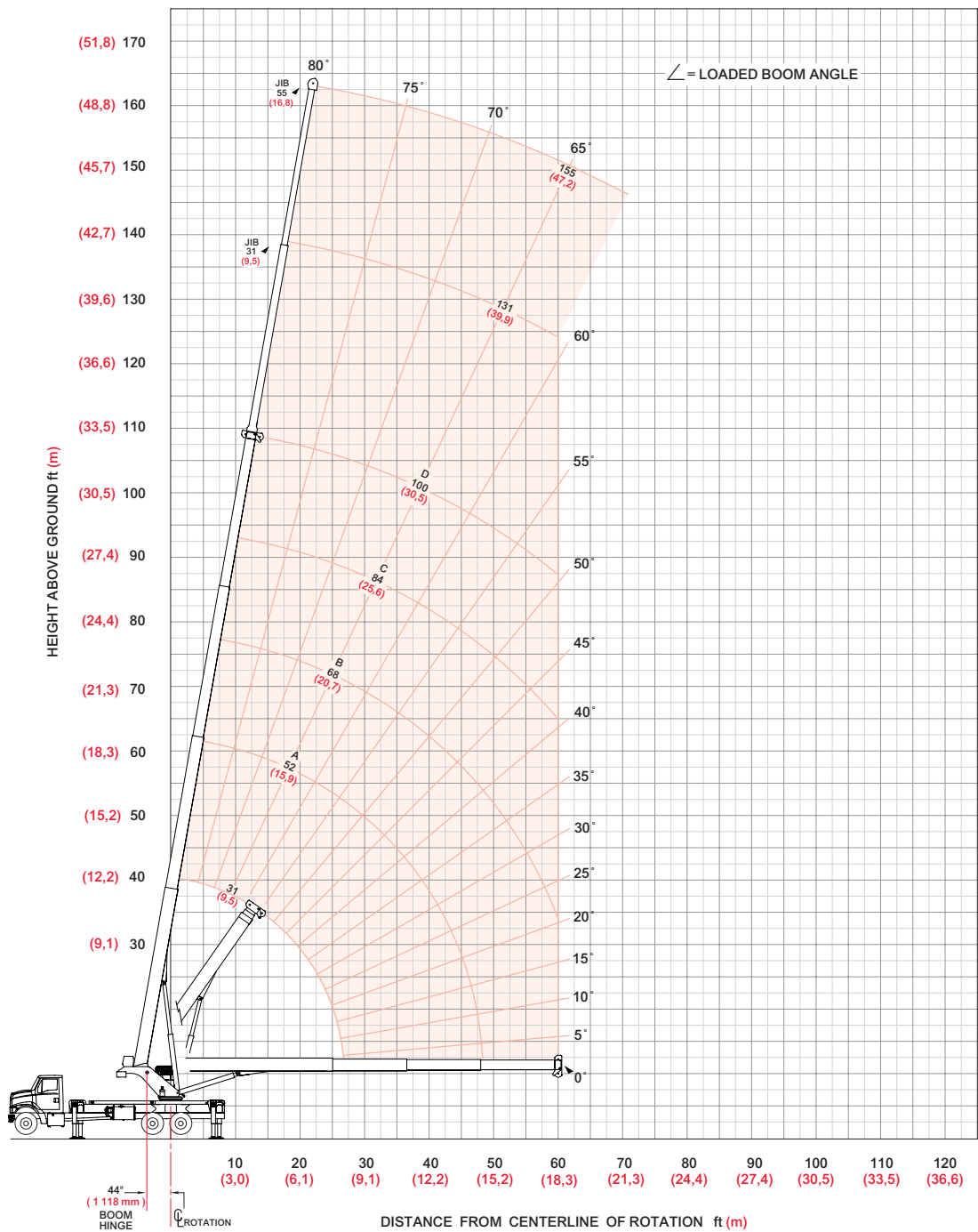
38100S Range Diagram - Intermediate
