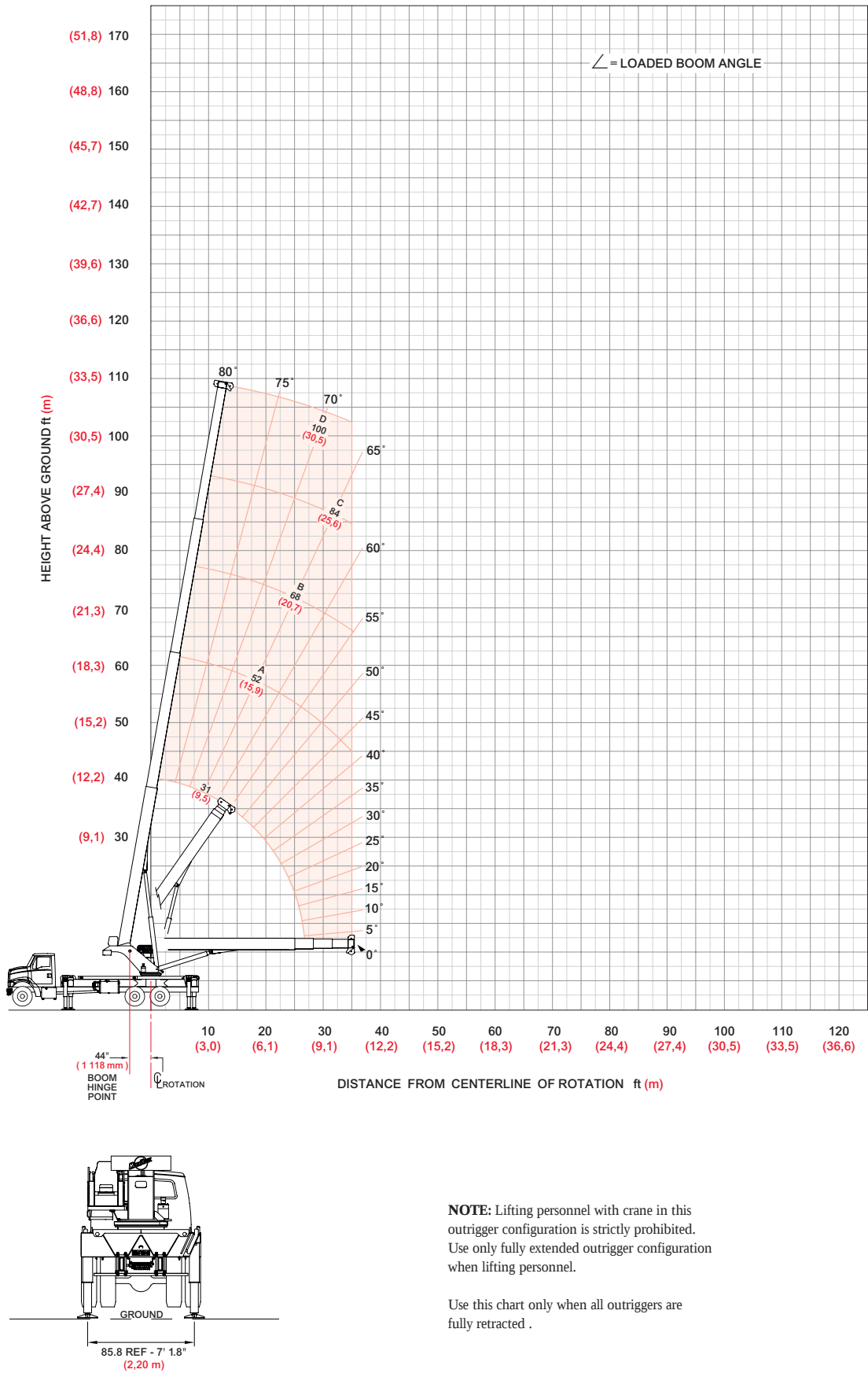
38100S Range Diagram - Fully Retracted
