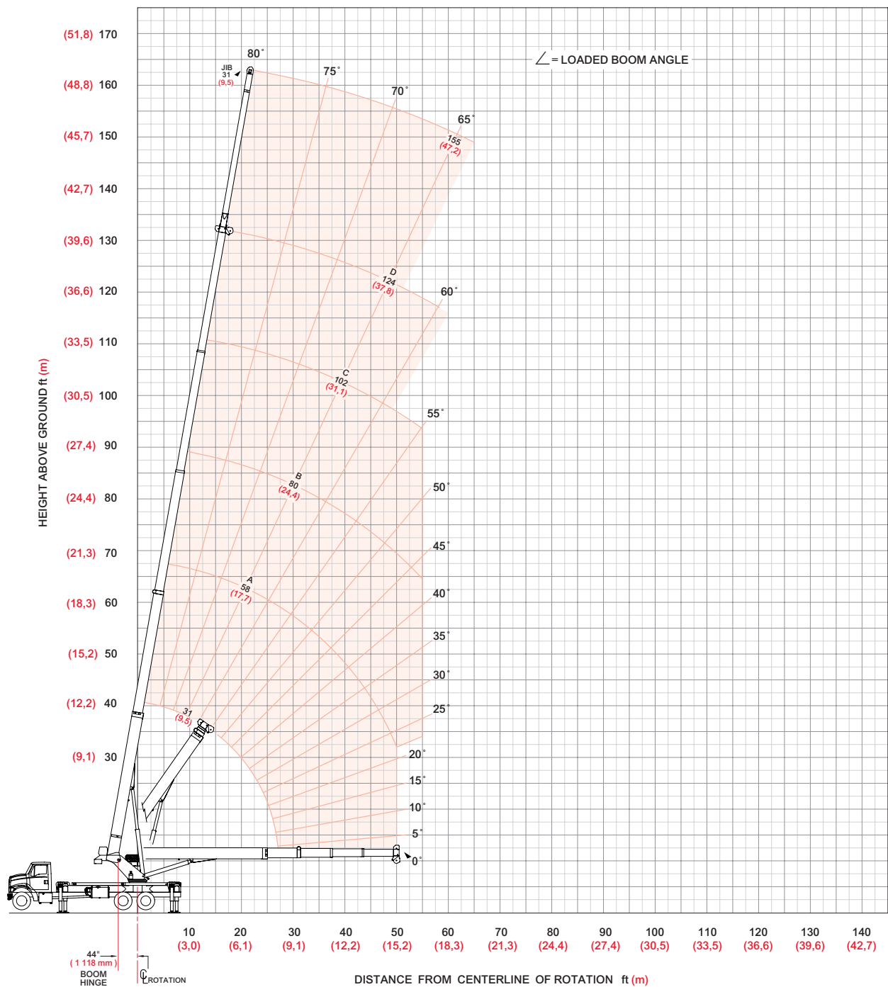
38124S Range Diagram - Intermediate
