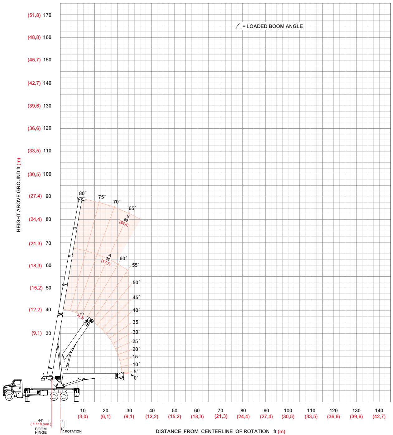
38124S Range Diagram - Fully Retracted
