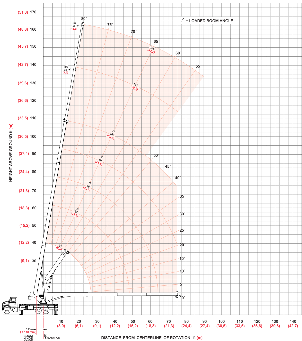
38100SHL Range Diagram - Intermediate
