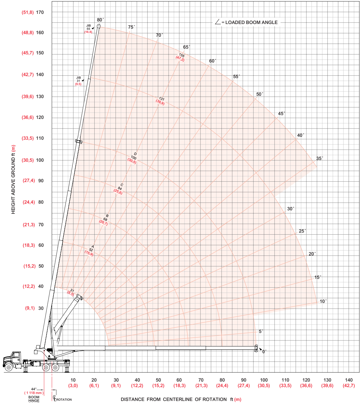
38100SHL Range Diagram - Fully Extended
