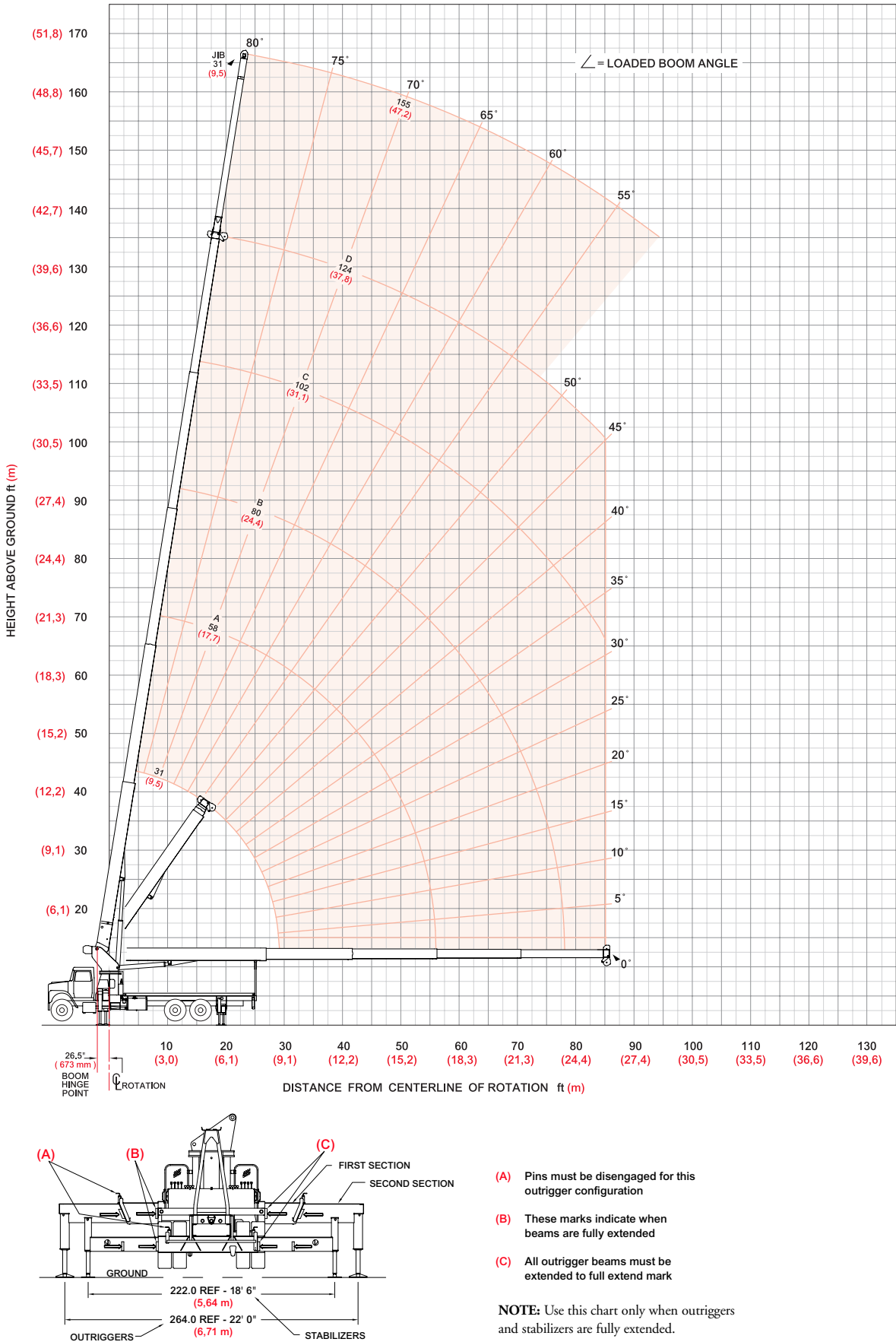
30124C Range Diagram - Fully Extended
