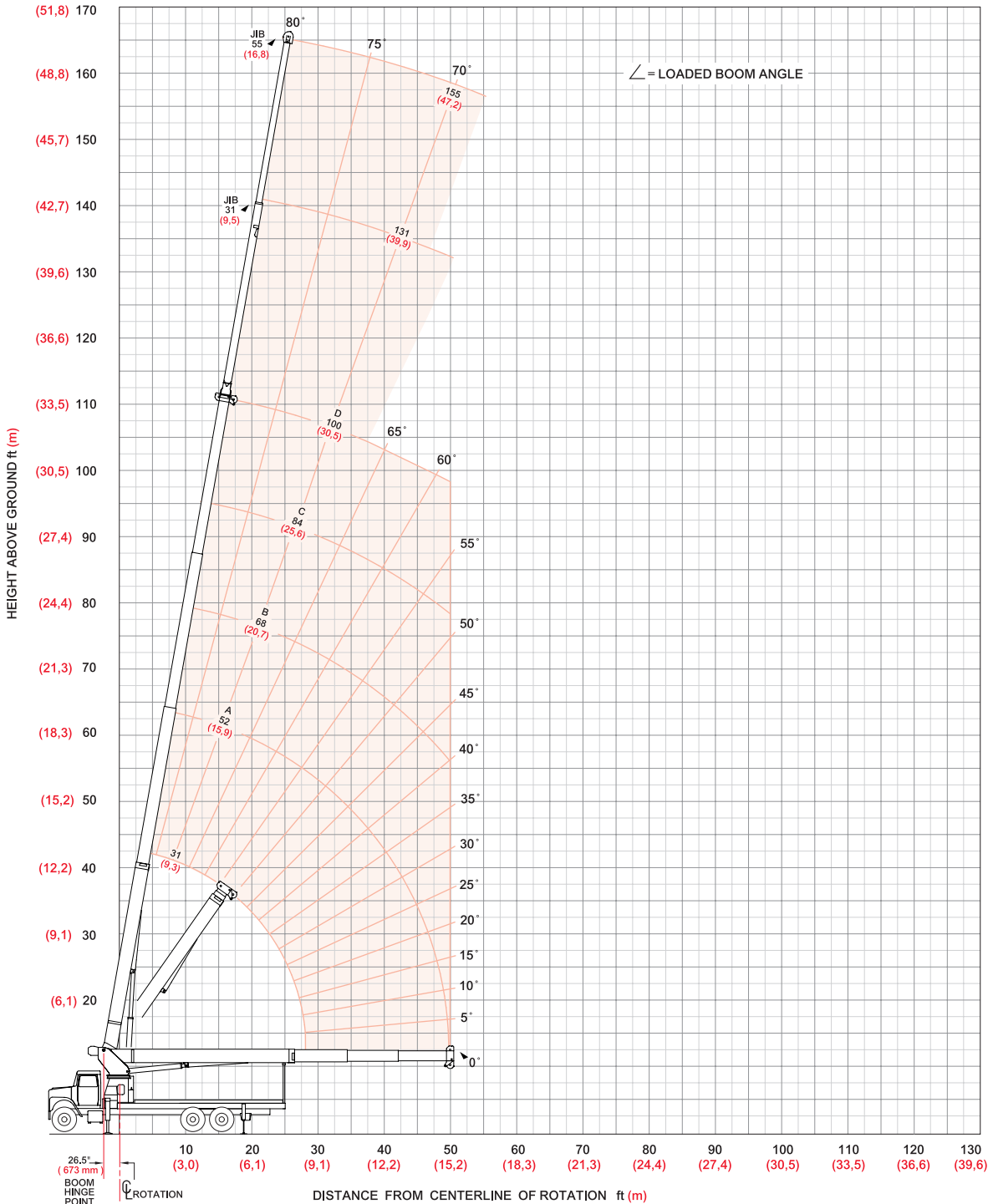
30100C Range Diagram - Intermediate
