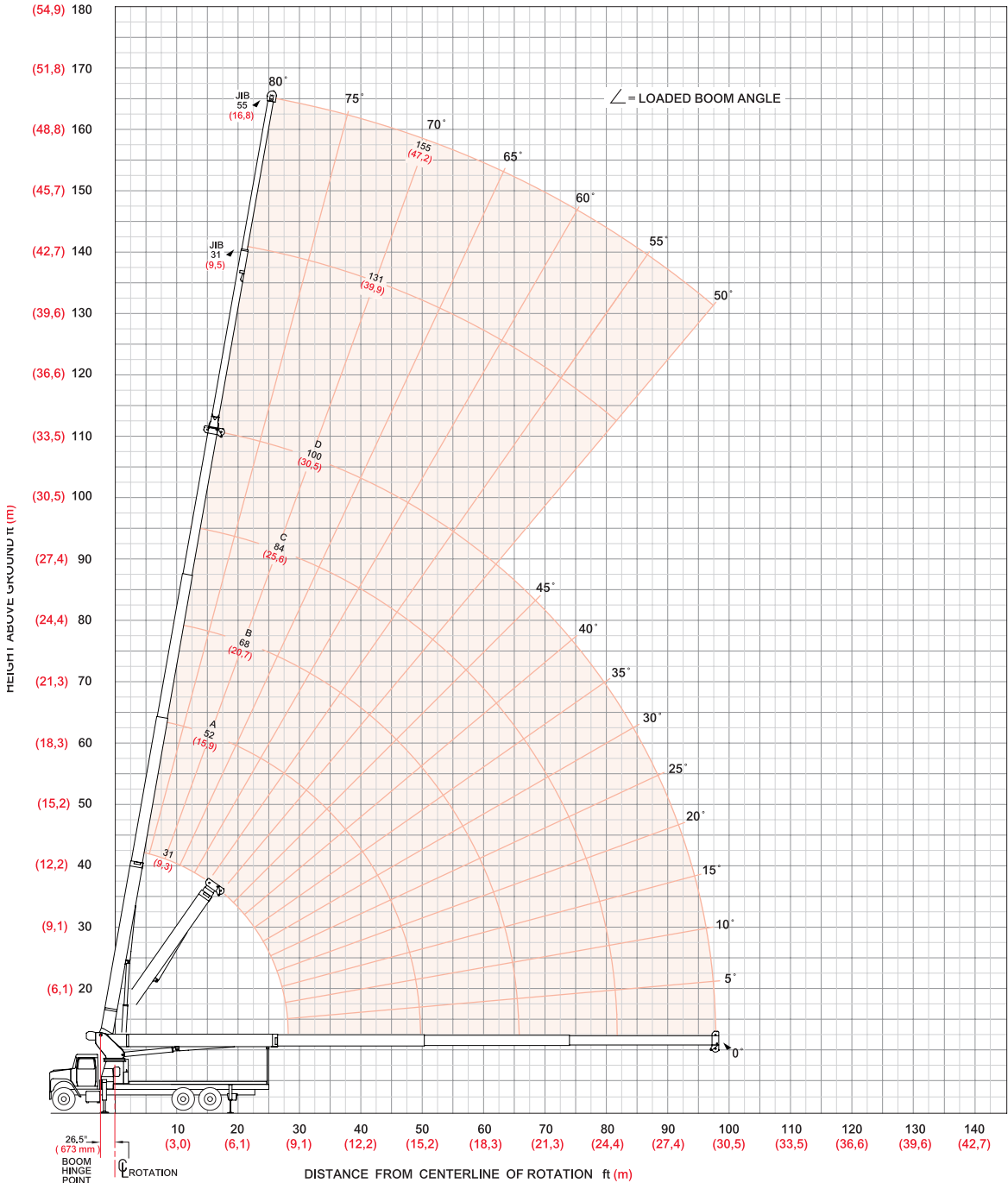
30100C Range Diagram - Fully Extended
