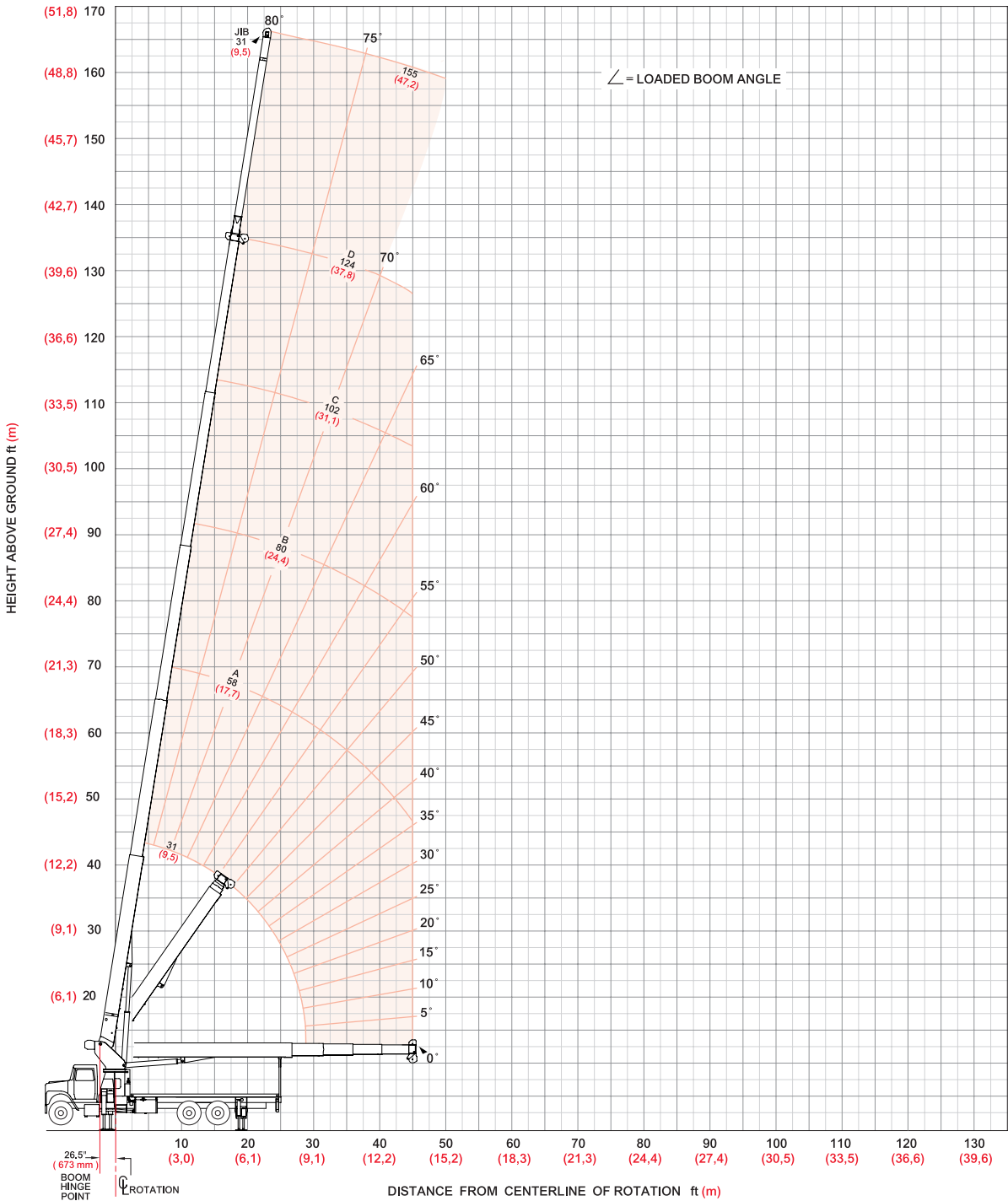
30124C Range Diagram - Intermediate
