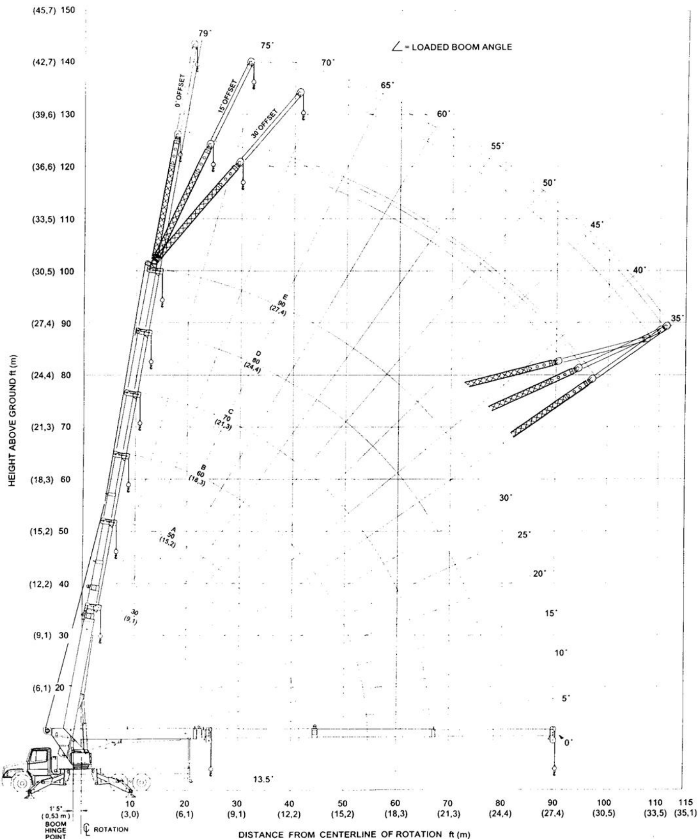
2892SX Range Diagram
