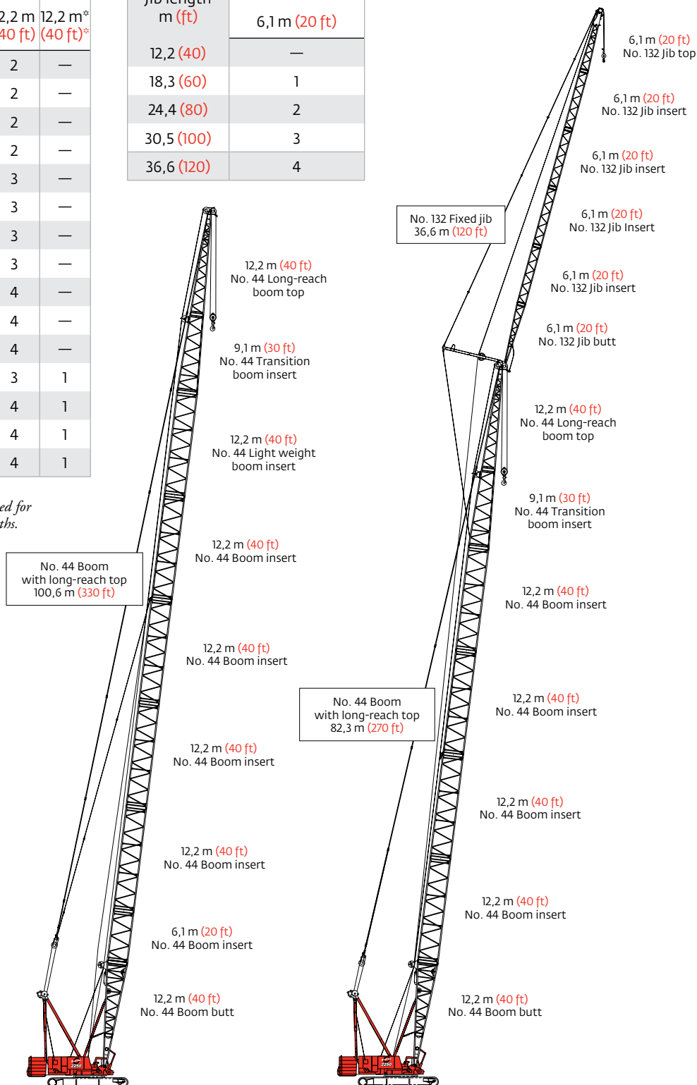
Model 2250 Series 3 No. 132 Fixed jib on No. 44 Main boom with long-reach top 118,9 m (390 ft)
