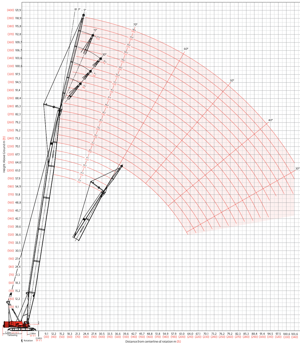
No. 132 Fixed jib on No. 44 Long-reach boom
