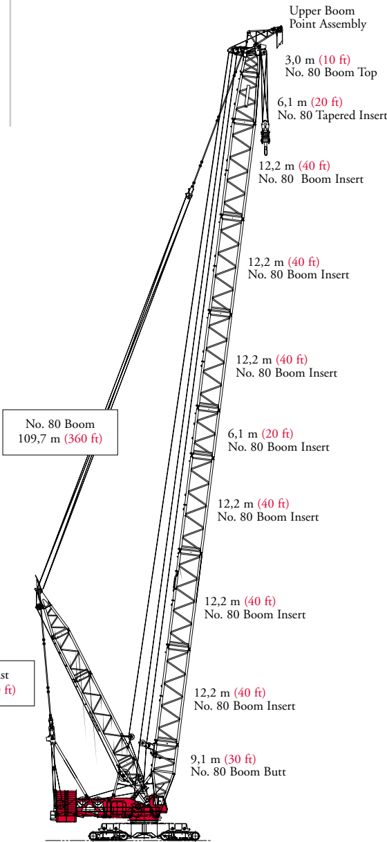
Model 21000 No. 80 Main Boom with No. 81 Mast 109,7 m (360 ft)
