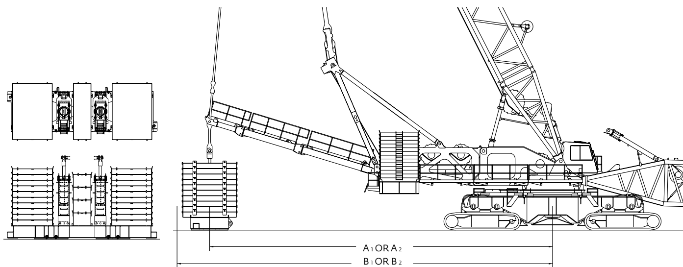
FREE HANGING COUNTERWEIGHT
