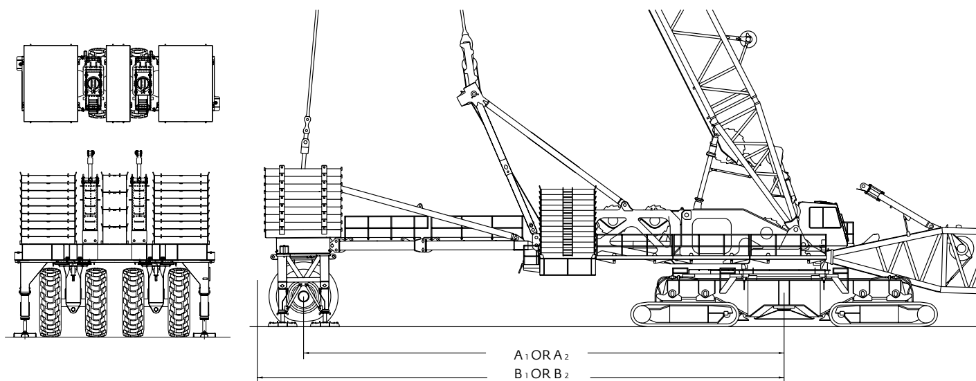
WHEELED COUNTERWEIGHT
