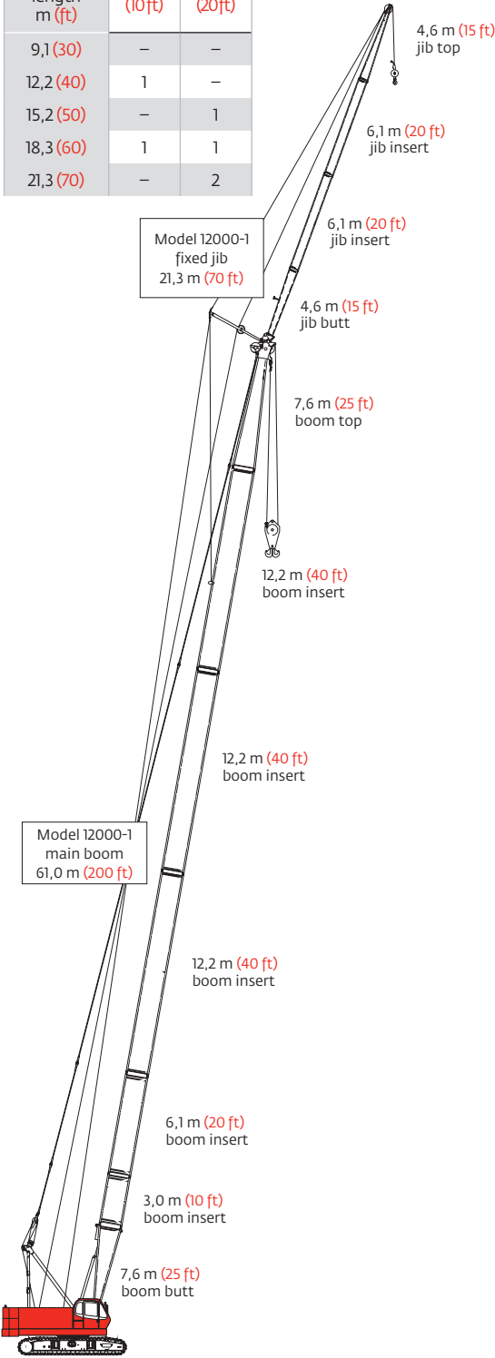
Model 12000-1 Fixed jib on main boom 82,3 m (270 ft)
